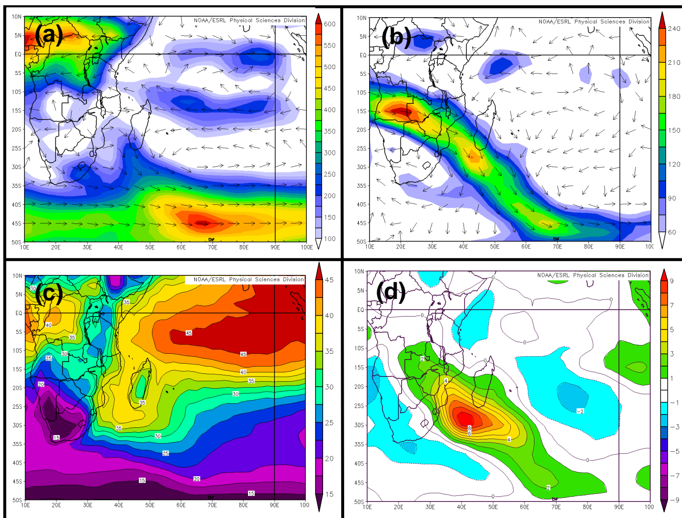
FIG. 8. Composite images of the 108 TME events, including: (a) 700-hPa moisture flux (shaded with vectors, (g\ kg^{-1}) \cdot (m\ s^{-1}) ), (b) 700-hPa moisture flux anomaly (shaded with vectors, (g\ kg^{-1}) \cdot (m\ s^{-1}) ), (c) PW (shaded, kg\ m^{-2} ), and (d) PW anomaly (shaded, kg\ m^{-2} ). Plumes of high precipitable water values extending poleward off the southeastern portion of Africa is a classic characteristic of TMEs in this region.
