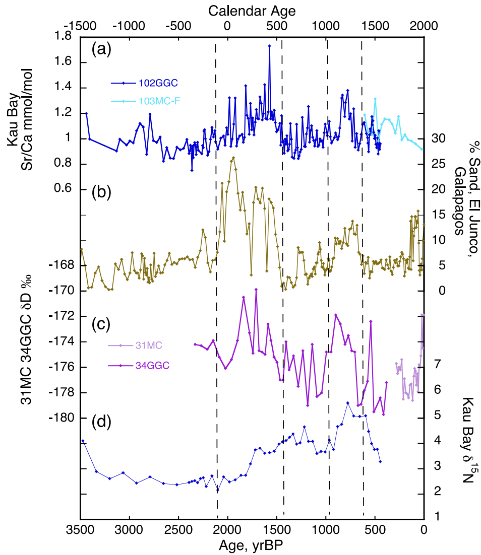
Figure 3.9. (a) Kau Bay C. acicula Sr/Ca, (b) El Junco % sand record (Conroy et al., 2008), (c) Makassar Strait \delta D (Tierney et al., 2010), and (d) Kau Bay \delta^{15}N (Langton et al., 2008). Dashed lines outline similarities between the records.
