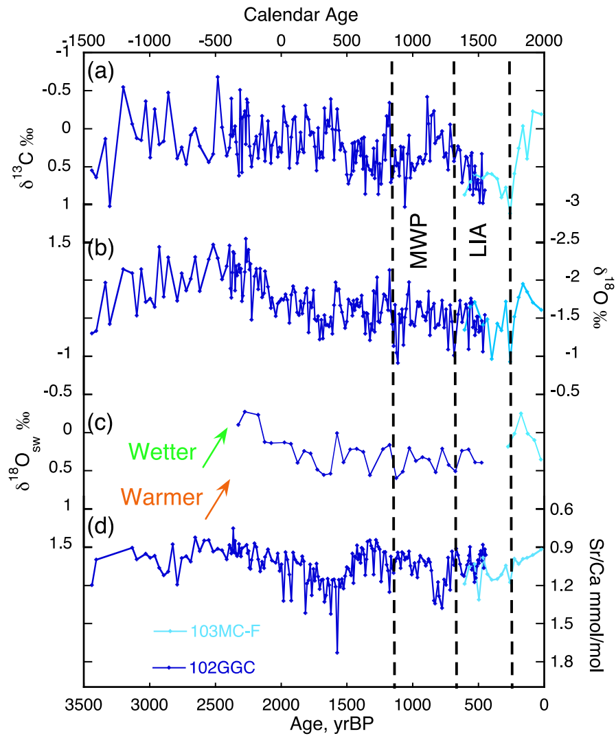
Figure 3.6. Data from Kau Bay cores 103MC-F and 102GGC. (a) C. acicula \delta^{13}\text{C} ; (b) C. acicula \delta^{18}\text{O} , (c) \delta^{18}\text{O}_{\text{sw}} generated from 50yr binned averages of SST from 31MC and 34GGC (Oppo et al. , 2009) and C. acicula \delta^{18}\text{O} (d) C. acicula Sr/Ca.
