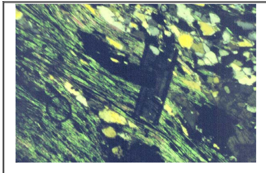
Figure 38: Crossed-polars photomicrograph from thin section BWH of a chloritoid crystal. Foliation, defined by muscovite, can be seen passing through chloritoid crystal indication crystal growth occurred after foliation development. Therefore: S1 → chloritoid. Chloritoid crystal is approximately 1mm in length.
