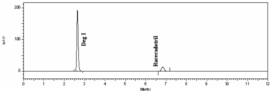
FIGURA 4. Cromatograma de HPLC de racecadotril con degradación oxidativa. FIGURE 4. HPLC chromatogram of oxidative degraded racecadotril.
