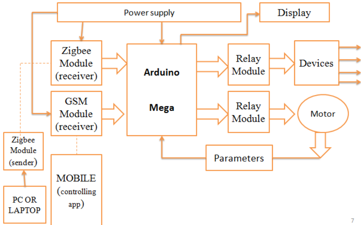
Figure 2: Block Diagram of Proposed System
