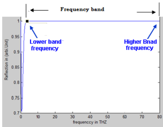
Fig2: Reflected band result for Mica SNG structure with respect to THz frequency.
