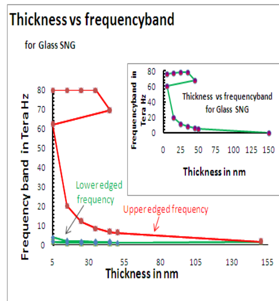
Fig 6: Result for lower reflected band, Higher reflected band and bandwidth DNG Mica grating structure.
