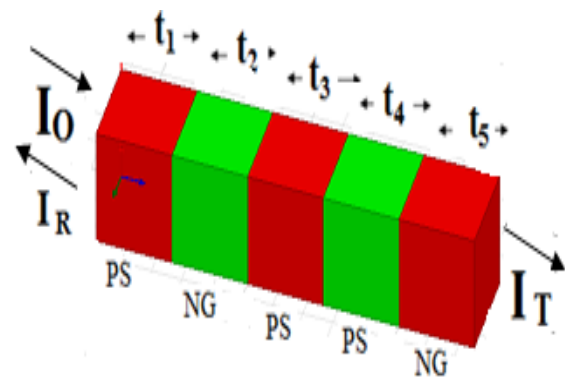
Fig1: Five layer Matamaterial structure
