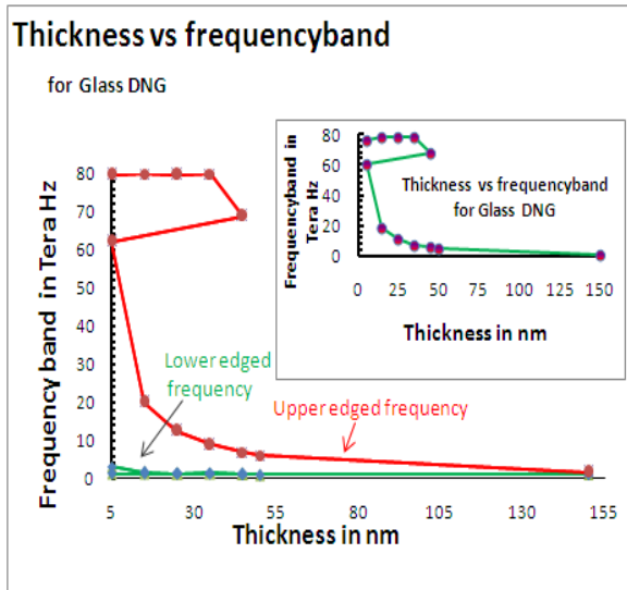
Fig 7: Result for lower reflected band, Higher reflected band and bandwidth DNG Glass grating structure.
