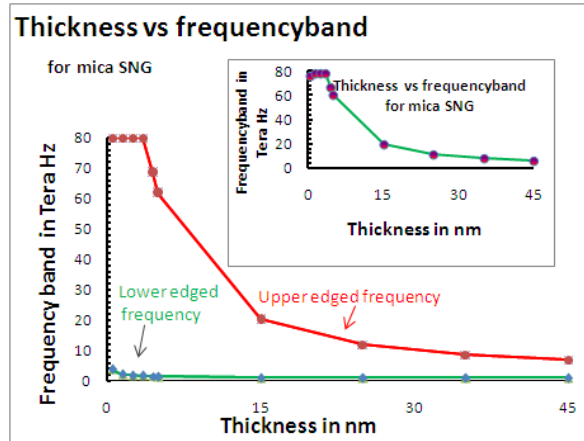
Fig 4: Result for lower reflected band, Higher reflected band and reflected bandwidth SNG Mica grating structure
