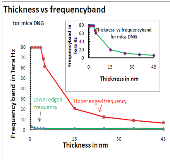
Fig 5: Result for lower reflected band, Higher reflected band and bandwidth DNG Mica grating structure.
