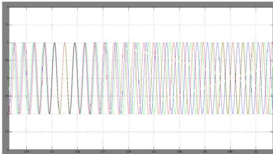
Fig16 Simulation waveform of unbalanced Three phase voltage
