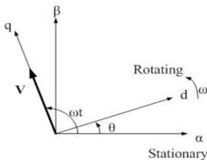
Fig4 Synchronous rotating reference frame
