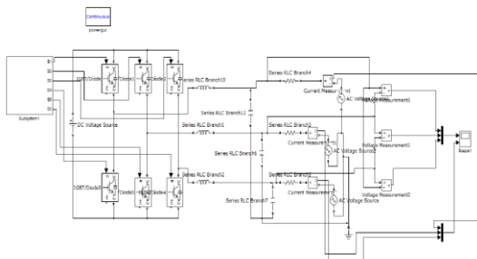
Fig10 Simulation diagram of grid connected 3 phase inverter
