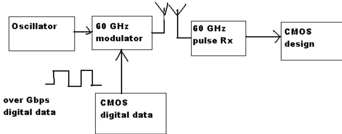
Fig: 2. Block diagram of 60 GHz channel modeling
