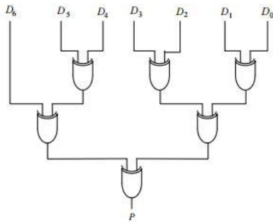
Fig. 7 Logic Circuit of Parity Bit Parameter Extractor
