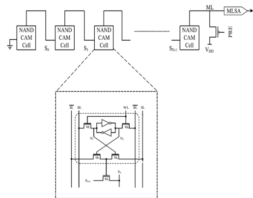
Fig. 2 Word Structure of NAND-Type CAM
