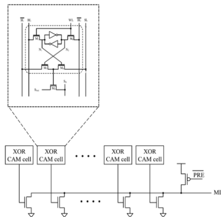
Fig. 3 Word Structure of NOR-Type CAM
