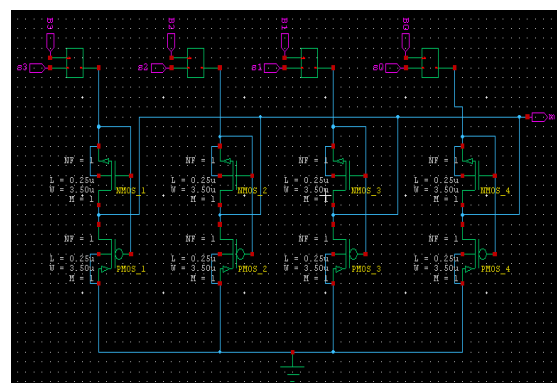
Fig. 11 Design of SCPF CAM
