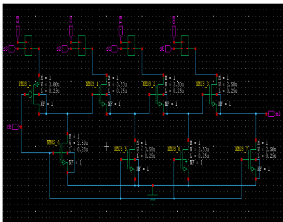
Fig. 8 Design of PF CAM
