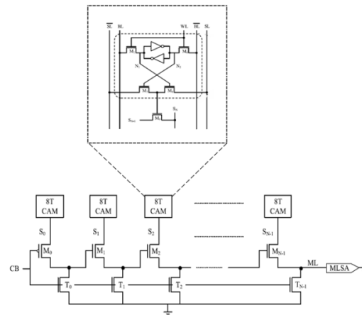
Fig. 4 Word Structure of PF CAM
