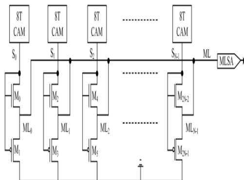
Fig. 5 Word Structure of SCPF-CAM
