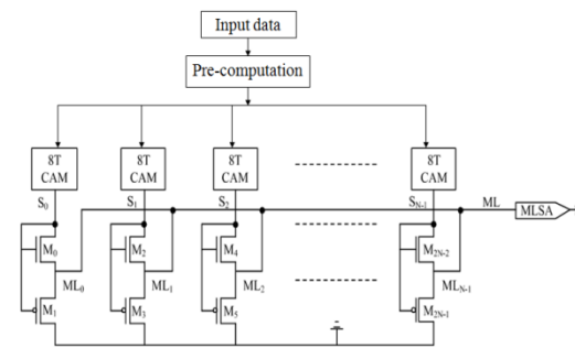
Fig. 6 Block Diagram of PB-SCPF CAM
