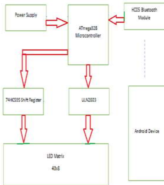
Fig. 1: Block Diagram.
