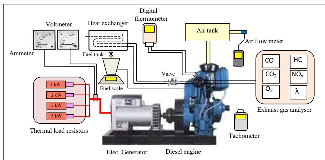
Figure 2: Schematic diagram of the diesel engine and instrumentation system.
