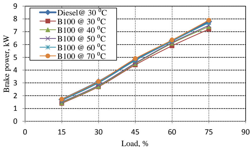
Figure 3: Output engine power at different loads.
