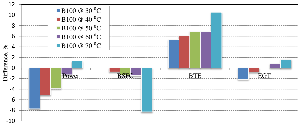
Figure 7: Differences in engine performance characteristics ( P_B , BSFC, BTE and EGT, in %) for the different inlet biodiesel and conventional diesel inlet temperatures (baseline: diesel fuel) at an engine load of 75 %.
