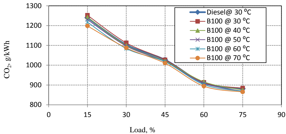
Figure 8: CO 2 emission of engine at different loads.
