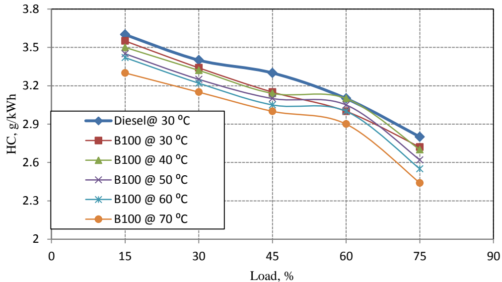
Figure 10: HC emissions from the engine at different loads.
