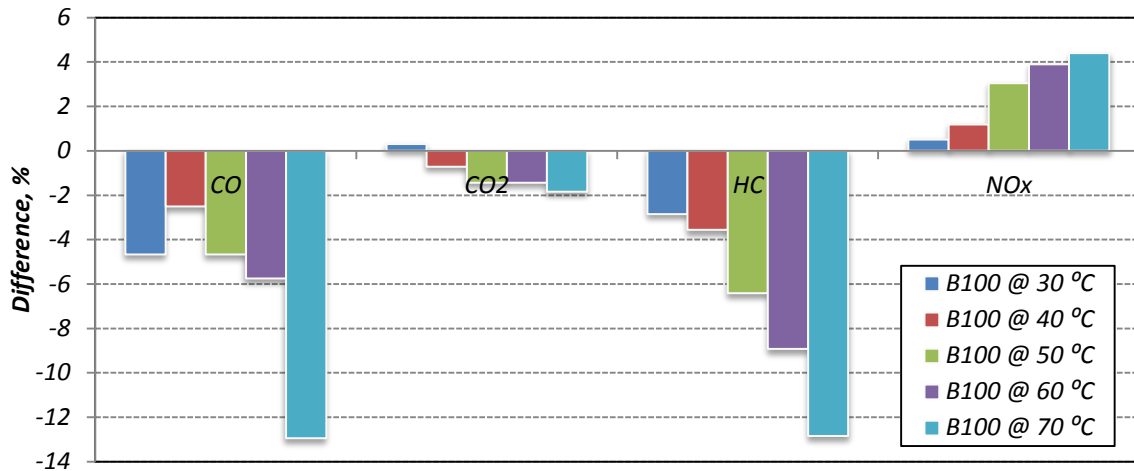
Figure 12: Difference percentages of the engine emission pollutants ( CO_2 , CO , HC and NO_x ) at different biodiesel and conventional diesel inlet temperatures (baseline: diesel fuel) at an engine load of 75 %.
