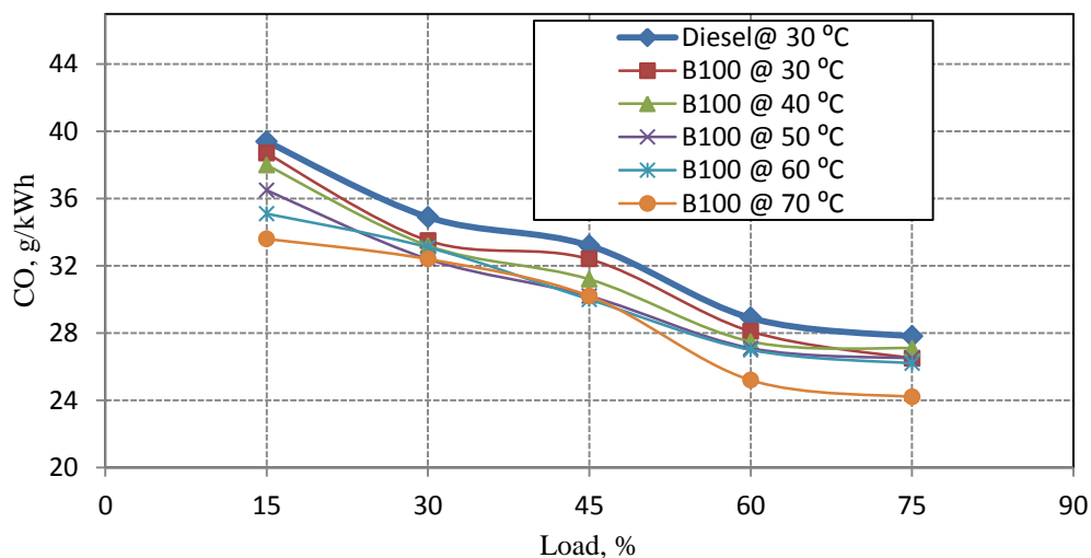
Figure 9: CO emissions from the engine at different loads.
