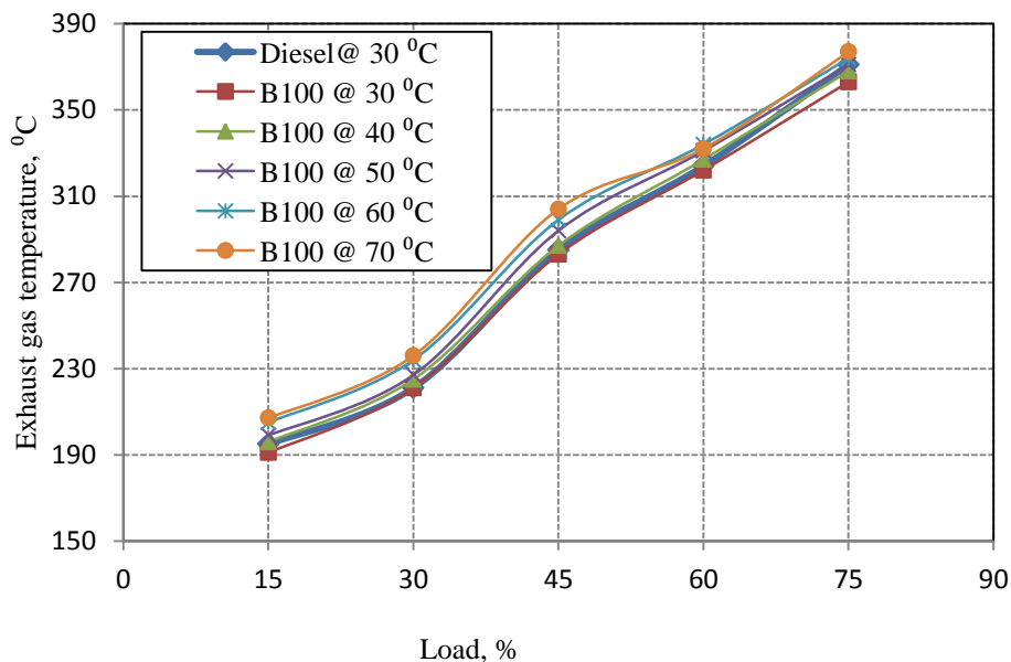
Figure 6: Exhaust gas temperature of the engine at different load.
