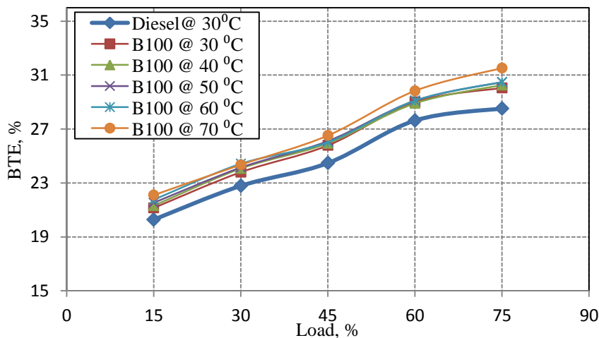
Figure 4: Brake thermal efficiency of the engine at different loads.
