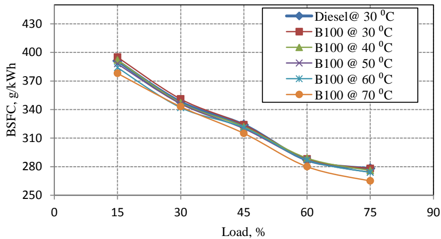
Figure 5: Brake specific fuel consumption of the engine at different loads.
