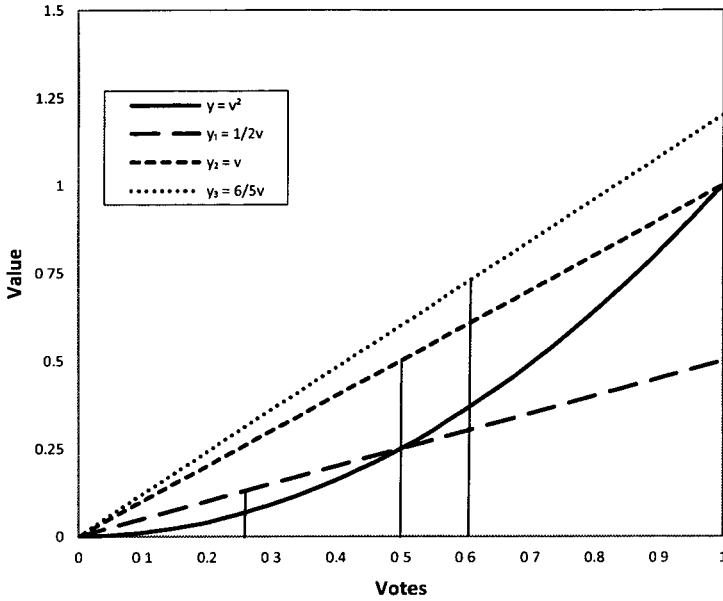
Figure 1: Relative Voting Power Under Quadratic Voting
