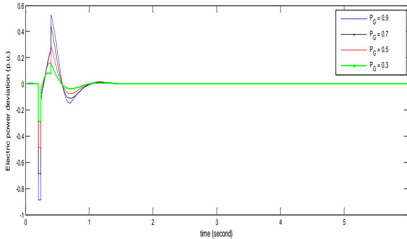
Figure 4.6: Effect of low to high generation power on the system electric power
