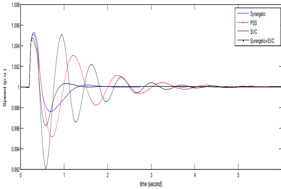
Figure 4.5: Speed of the generator
