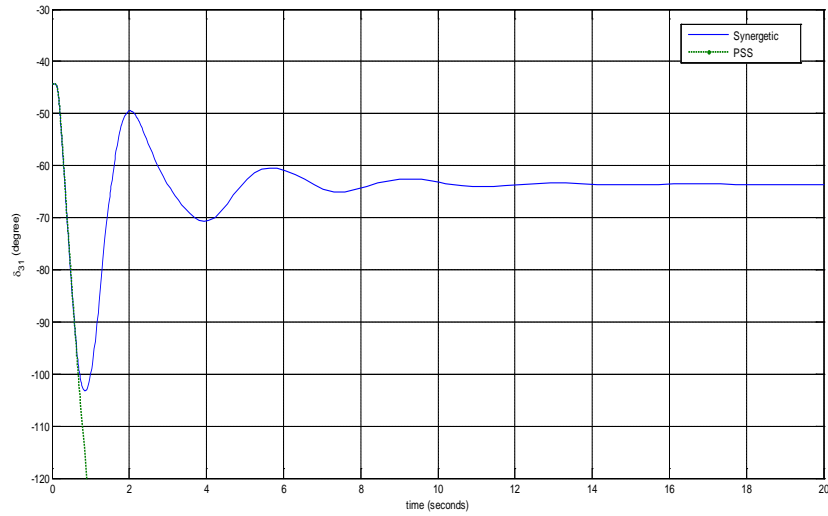
Figure 3.25: Relative rotor angle (degree) 3 - 1 for case II (TAS)
