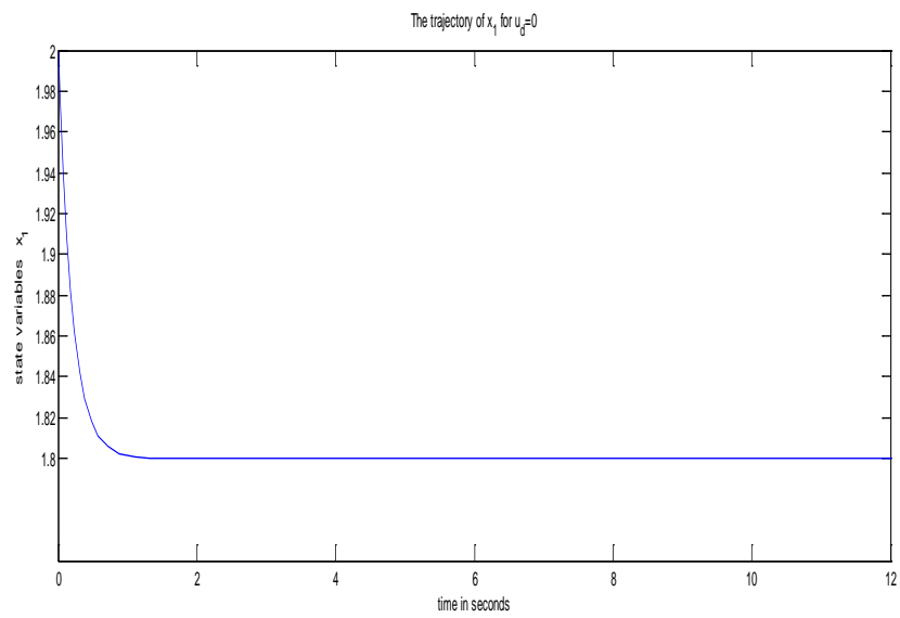
Figure 3.4b: Variable x_1 for \eta = 0
