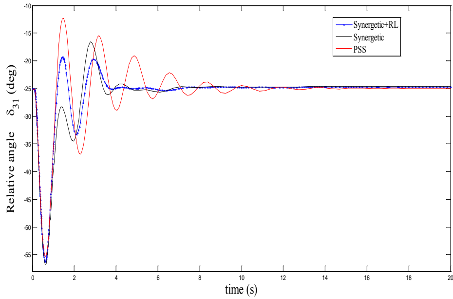
Figure 5.2: Relative angle \delta_{31} under Operating Condition I
