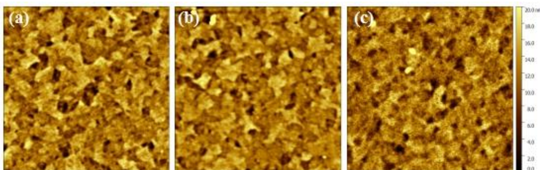
Figure 5.3 AFM scans of 100 nm CBP films over a 5 \mu\text{m} \times 5 \mu\text{m} area. Film (a) was undoped, film (b) was doped with 30mol% WO 3 by co-deposition and film (c) was doped by sequential deposition of alternative 0.5 nm WO 3 and 3 nm CBP layers.
