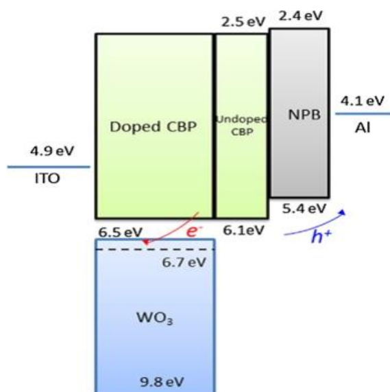
Figure 4.5 Energy diagram of hole-only device with a WO 3 -doped CBP HTL.
