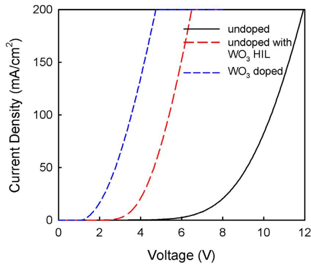
Figure 4.9 J-V characteristics of hole-only devices with a HTL comprising 100 nm undoped CBP, 100 nm 30mol% \text{WO}_3 -doped CBP, or 0.5 nm \text{WO}_3 / 100 nm undoped CBP.
