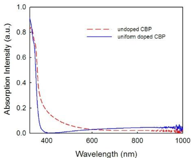
Figure 4.6 Absorption of thin film comprising 100 nm 30mol% WO 3 doped CBP and 100 nm undoped CBP
