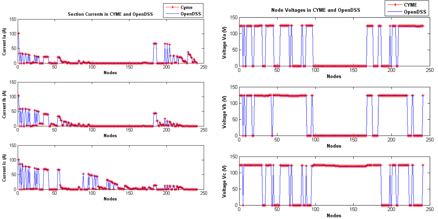
Figure 5-4 (a)-(b) Section Currents and Node Voltages in CYMDIST and OpenDSS
