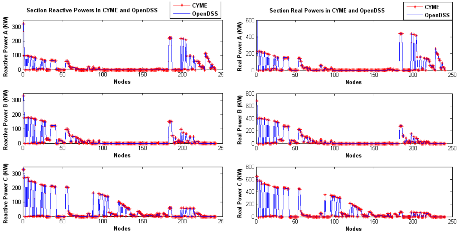
Figure 5-5 (a)-(b) Real and Reactive powers through a section in CYMDIST and OpenDSS
