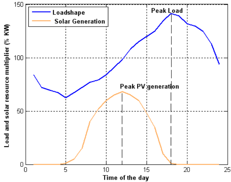
Figure 5-9 Time Varying PV and load profiles
