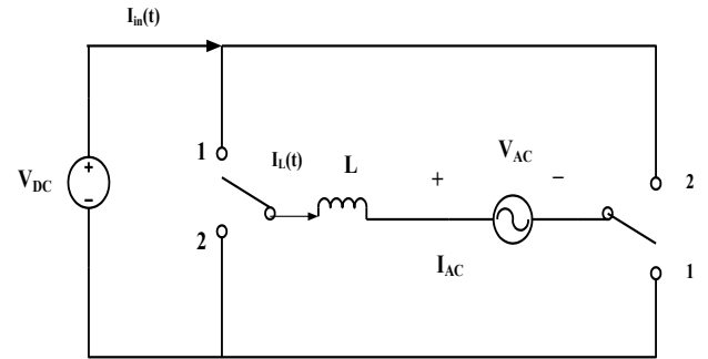
Figure 4-12 DC-AC Inverter Model.
