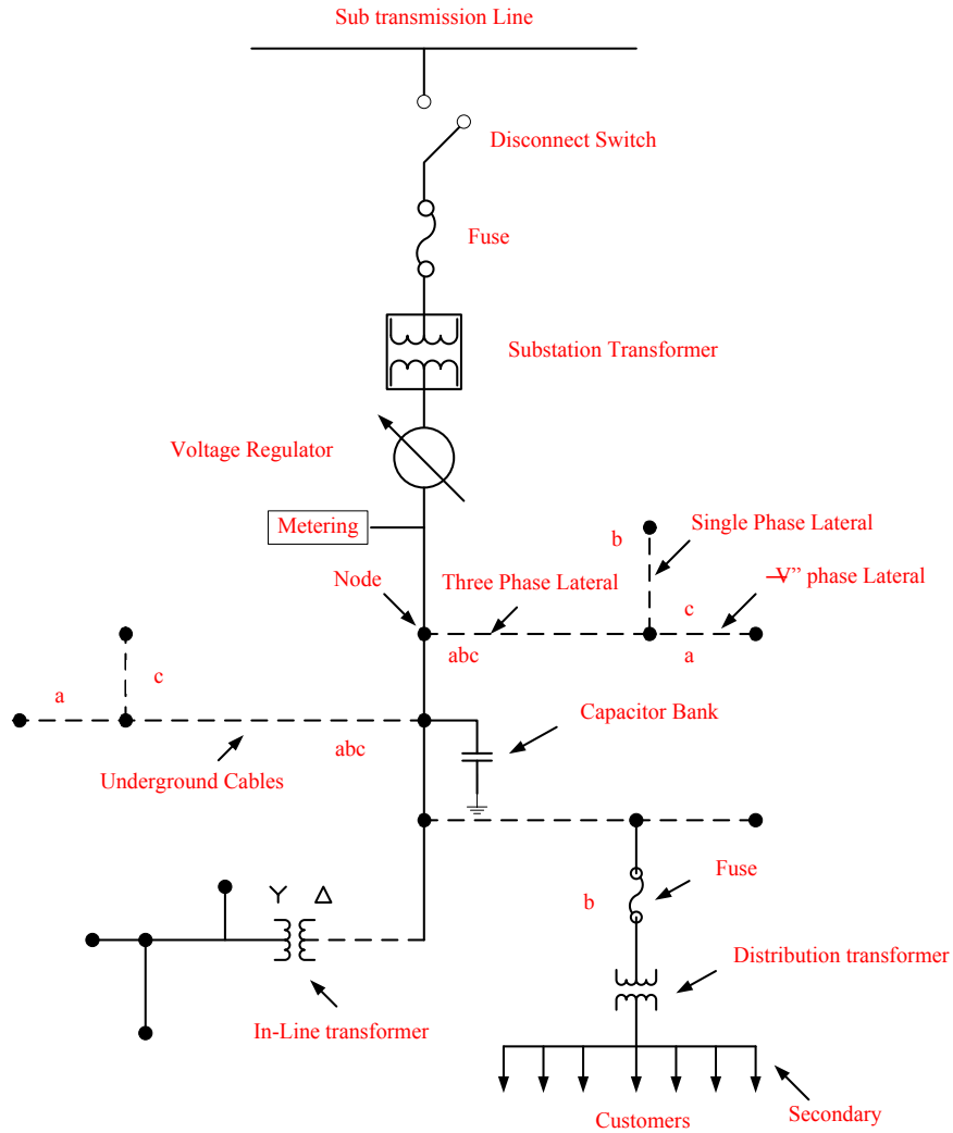
Figure 1-1 Simple Distribution Feeder [4]
