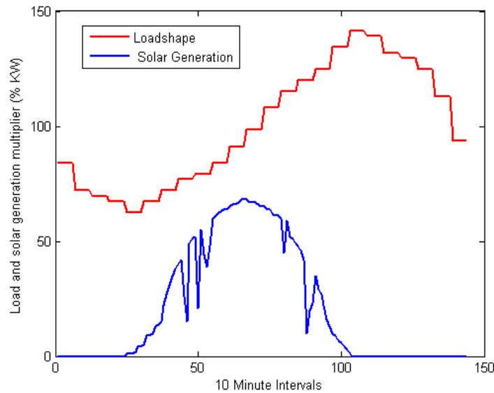
Fig. 5-14: 10-minute varying PV and load shapes to simulate cloud cover
