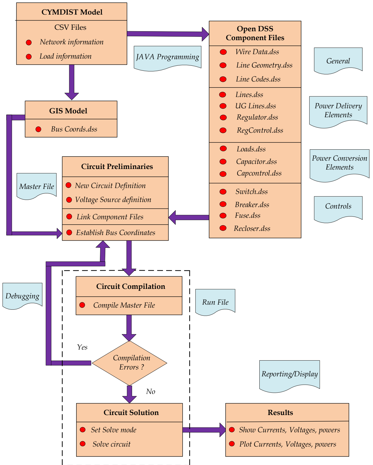
Figure 5-1 Final Feeder Data Model Conversion in OpenDSS
