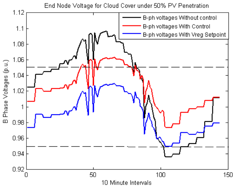
Fig. 5-16 End node voltages with 50% PV penetration under a cloud cover scenario.
