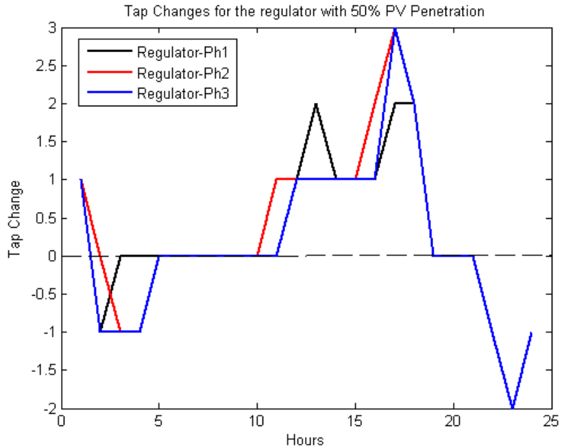
Figure 5-12: 24-hour Three phase Regulator tap changes
