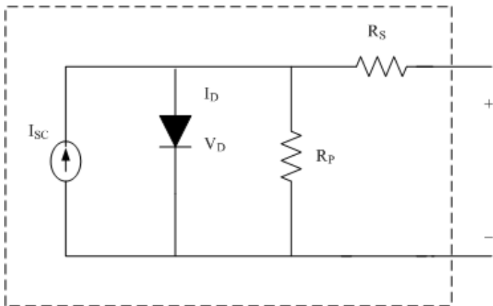
Figure 4-9 Individual PV Cell
