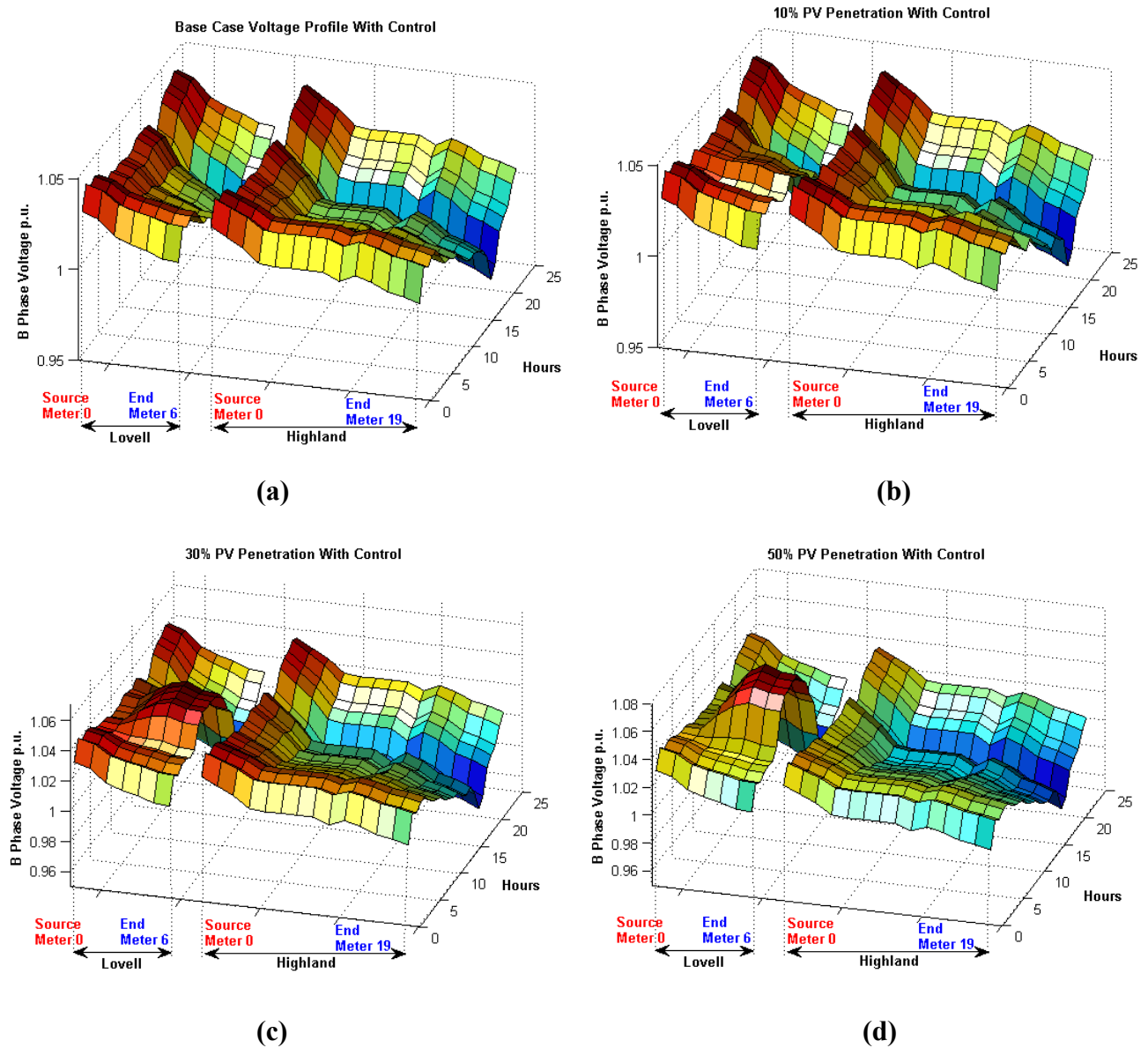
Fig. 5-10: Voltage profile of the circuit with controls (a): Base case (b) 10% PV penetration (c) 30% PV penetration (d) 50% PV penetration
