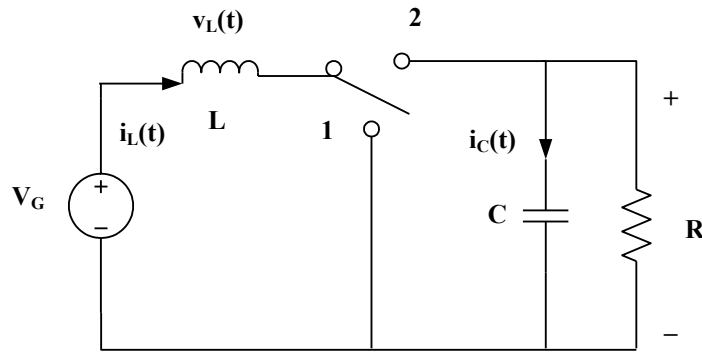
Figure 4-11 DC-DC Booster Model.
