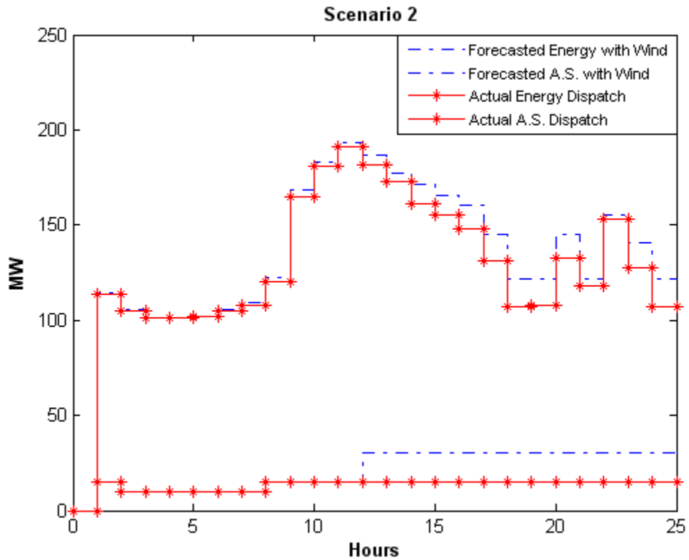
Fig.5-22 Bidding Strategy for Scenario II
