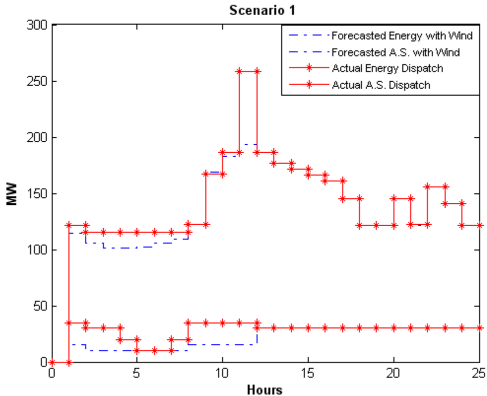
Fig.5-21 Bidding Strategy for Scenario I
