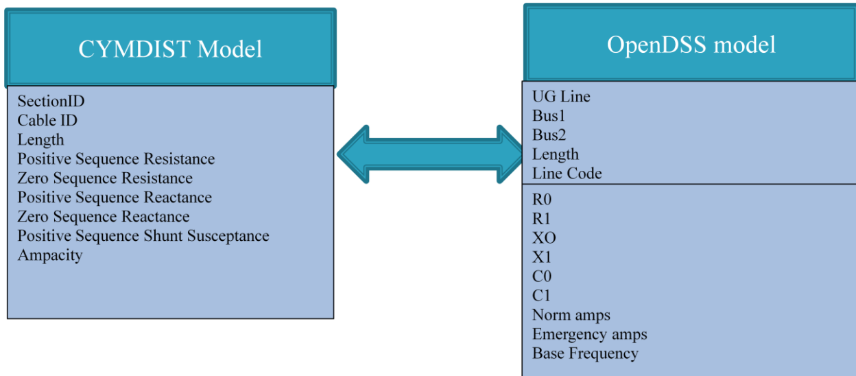
Figure 4-3(b) Comparison of the CYMDIST and OpenDSS models for underground lines.
