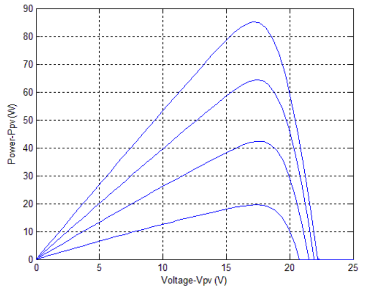
Figure 4-13(a) V-I characteristics for insolation ranging from 0.25 \text{ W/m}^2 to 1 \text{ W/m}^2 ; Figure 4-13(b) V-P characteristics for insolation ranging from 0.25 \text{ W/m}^2 to 1 \text{ W/m}^2
