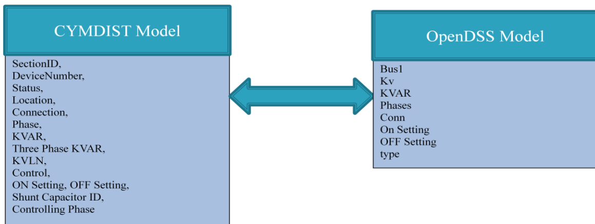
Figure 4-8 Comparison of the CYMDIST and OpenDSS models for Capacitor.
