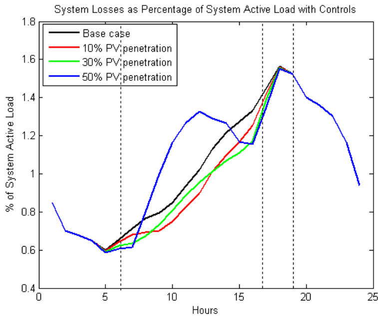
Fig. 5-13: Percentage System losses for various penetration levels
