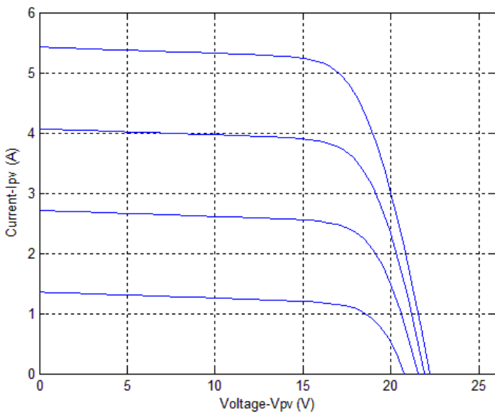
Figure 4-13(a) V-I characteristics for insolation ranging from 0.25 \text{ W/m}^2 to 1 \text{ W/m}^2 ; Figure 4-13(b) V-P characteristics for insolation ranging from 0.25 \text{ W/m}^2 to 1 \text{ W/m}^2
