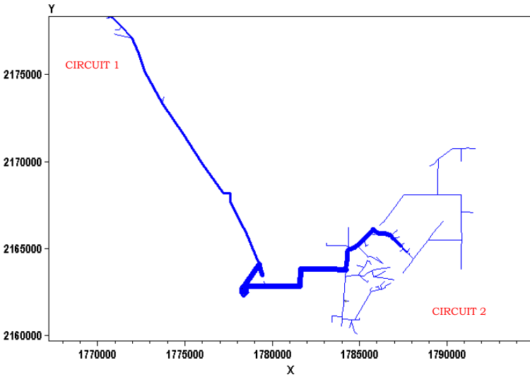
Figure 5-3 OpenDSS power flow plot for Feeder 2
