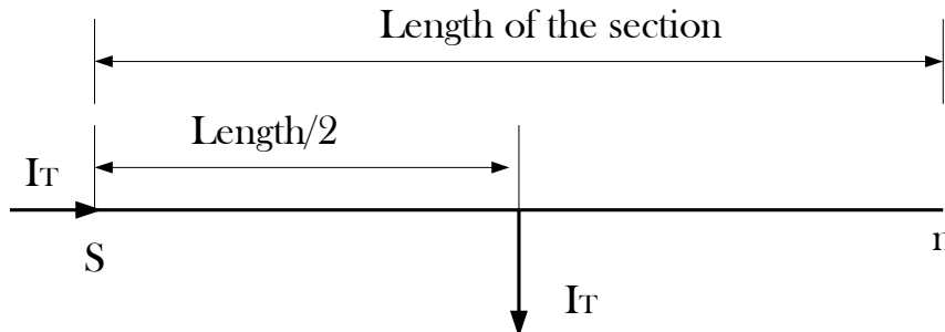
Figure 4-5 Distributed Load Model in OpenDSS.
