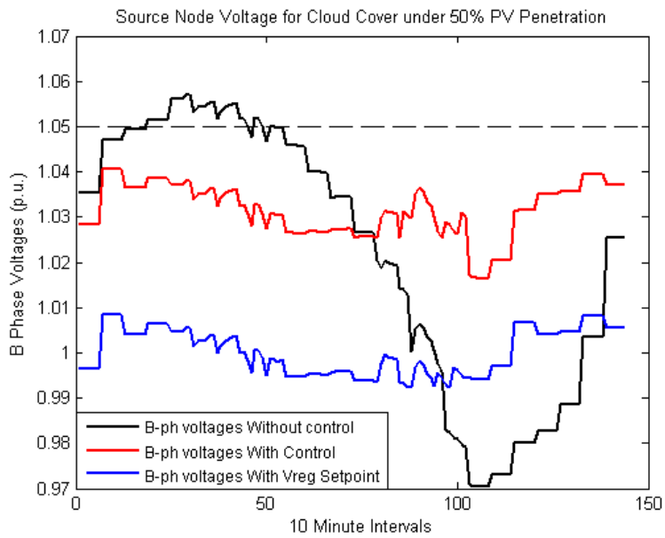
Fig. 5-15 Source node voltages with 50% PV penetration under a cloud cover scenario
