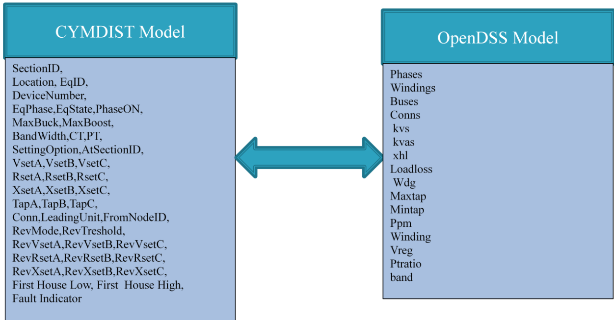
Figure 4-7 Comparison of the CYMDIST and OpenDSS models for Regulator.
