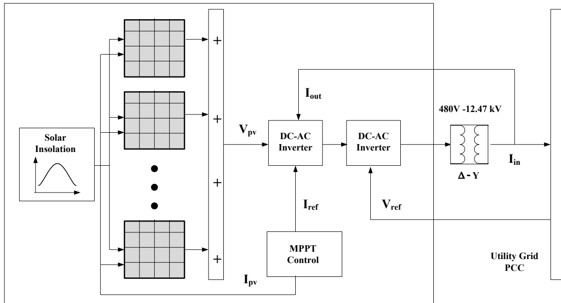
Figure 4-14 Utility scaled PV plant with interconnection transformer.
