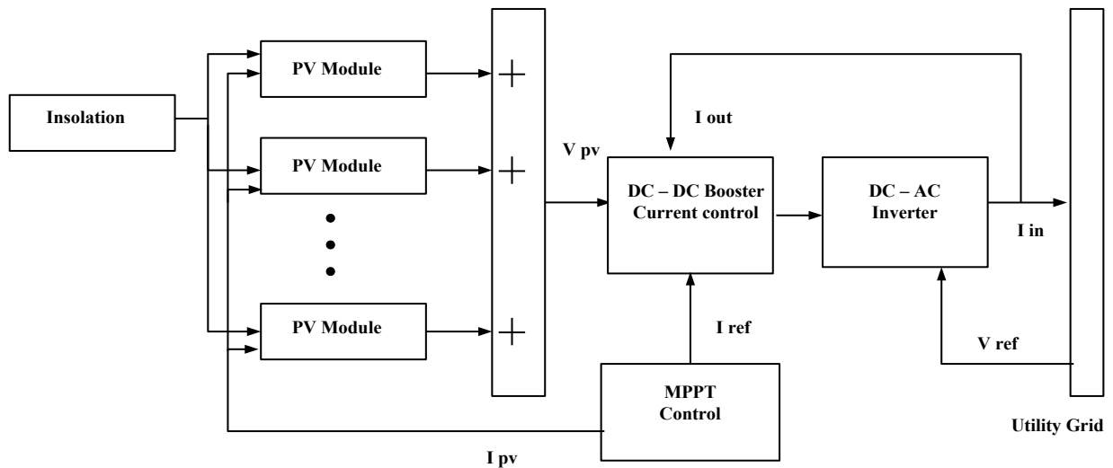
Figure 4-10 Grid Connected PV system.
