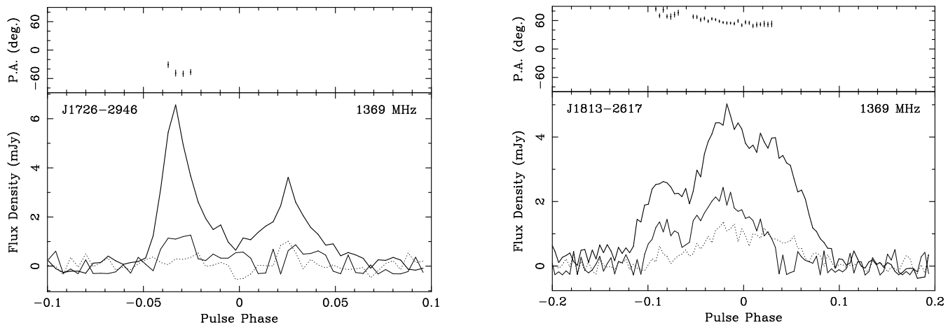
Figure 2. Integrated polarization profiles for the two MSPs for which significant RMs were detected. The top panels of each plot show the polarization position angle as a function of pulse phase. The bottom panels show total intensity (bold line), linear polarization (solid line) and circular polarization (dotted line).
