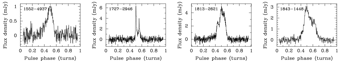
Figure 1. Integrated pulse profiles each showing 360 degrees of rotational phase at 20 cm wavelength for the four MSPs described in this paper. Data were obtained with the Parkes digital filterbank systems.
