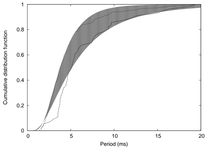
Figure 7. Cumulative distribution functions showing the observed sample of 56 MSPs (rightmost dashed curve), the 95% credible region of our best fitting log-normal model (shaded band) and the current sample of 206 MSPs with P < 20 ms (leftmost dashed curve). The deviation between the shaded band and the rightmost dashed curve highlights the observational selection effects at short periods in our sample of 56 MSPs.
