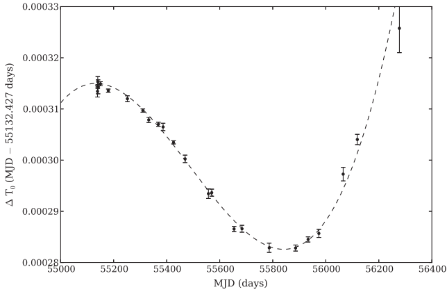
Figure 8. A plot of \Delta T_0 as a function of time for PSR J1731–1847. The dashed line shows the best-fitting curve from the timing solution generated with the BTX model in TEMPO2, employing up to the second orbital frequency derivative terms.
