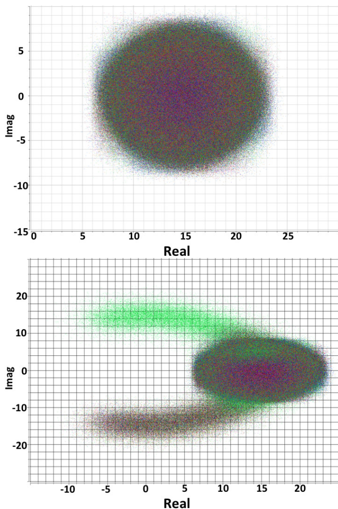
Fig. 3. Example of diagnostic plots during the calibration process (taken from Bühr 2016 ). The imaginary part of the visibility is plotted as a function of the real part for the calibrator 3C 286 in the HI line. The color-coding corresponds to the different antennas. For a point source like the calibrators a roundish cloud as shown in the top panel is expected. The deviations in the bottom panel isolate bad antennas that need to be flagged.
