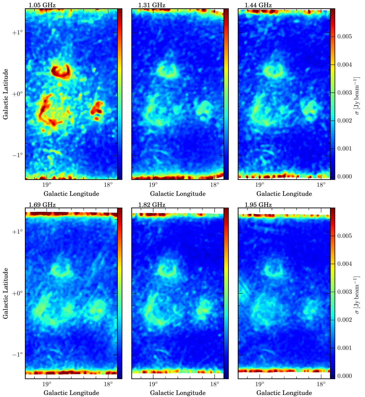
Fig. A.1. Example continuum noise maps in the 18 to 19 deg field. The scale bars for all wavelengths are the same. The frequencies increase from the top left to the bottom right corner . The noise level clearly depends on the source structure and the different bands.
