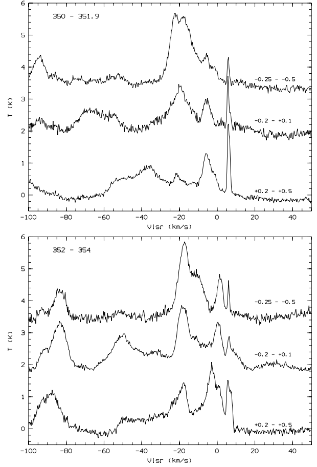
Fig. A.2. ^{12}\text{CO} average profiles extracted from ThrUMMS data cubes. The profiles are averaged over b = -0.25^\circ to -0.5^\circ ( top ), b = -0.2^\circ to +0.1^\circ ( middle ) and b = 0.2^\circ to 0.5^\circ ( bottom ) and l = 350^\circ to 351.9^\circ and l = 352^\circ to 354^\circ , respectively. The profiles are vertically-shifted from each other to better compare them.
