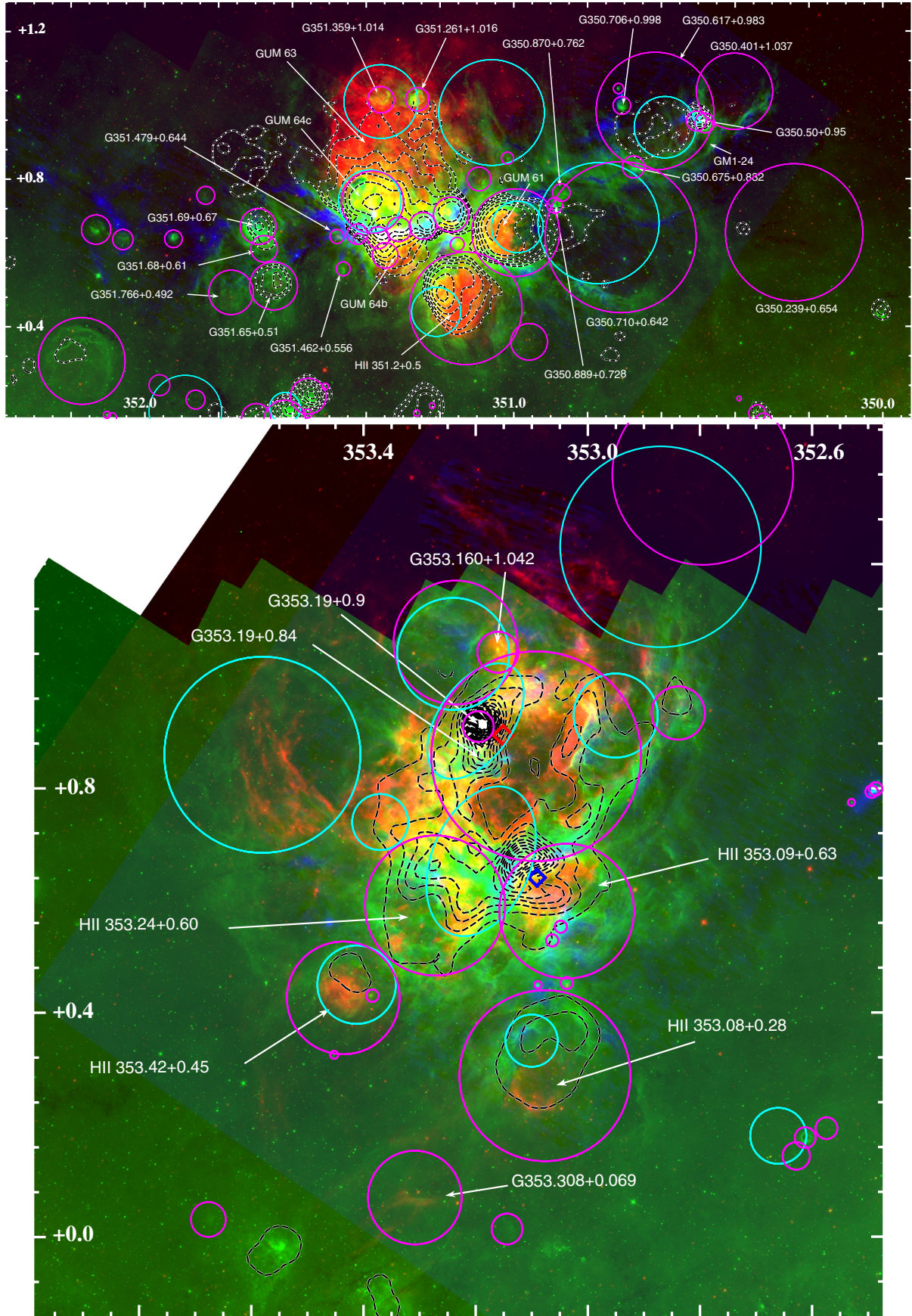
Fig. 1. H \alpha (red), GLIMPSE-8 \mu m (green), and SIMBA-1.2 mm (blue) composite image of NGC 6334 (upper panel) and NGC 6357 (lower panel). The quoted coordinates are galactic coordinates. The overlaid isocontours are from SGPS radio emission. The purple and cyan circles show the H II regions from Anderson et al. (2014) and Langston et al. (2000) respectively. For NGC 6357, the position of stellar clusters Pismis 24 (red diamond) and AH03J1725-34.4 (blue diamond) are also indicated.
