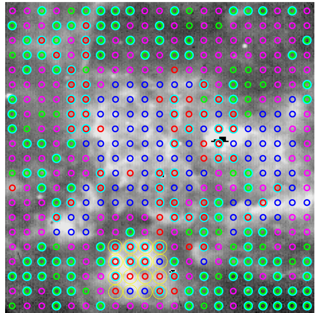
Fig. 12. Same as Fig. 10, but for the central part of NGC 6357. The points overlaid with circles belong to H II 353.09+0.63. In this field 34% of the profiles show \sigma > 10 \text{ km s}^{-1} .
