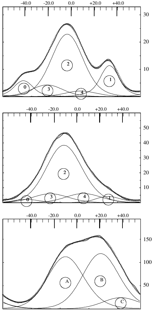
Fig. 4. Examples of H \alpha profile decomposition. The x -axis is the V_{\text{LSR}} (in \text{km s}^{-1} ) and the y -axis is the intensity (in arbitrary units). The geocoronal H \alpha and OH night-sky lines are the components noted 1 and 0, while the nebular lines are noted from 2 to 4 (their sum is the square-dotted line). The lower panel shows, as an example, the profile from GUM 61 central area (see text).
