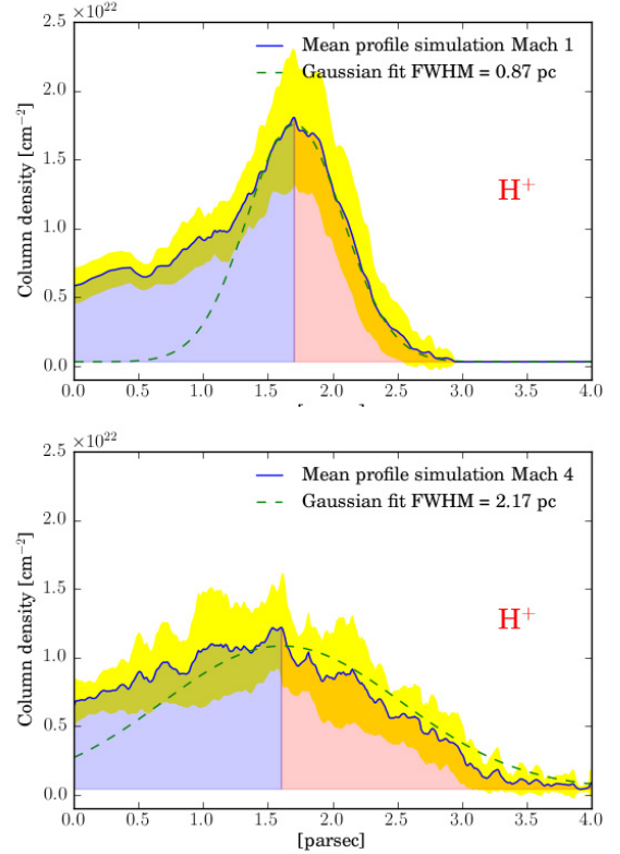
Fig. 12. Column density profiles of the two simulations shown in Fig. 11 after 1 My. The red sign H + indicates the position of the ionized gas in the simulation. The flux is coming from the right side of the profiles.
