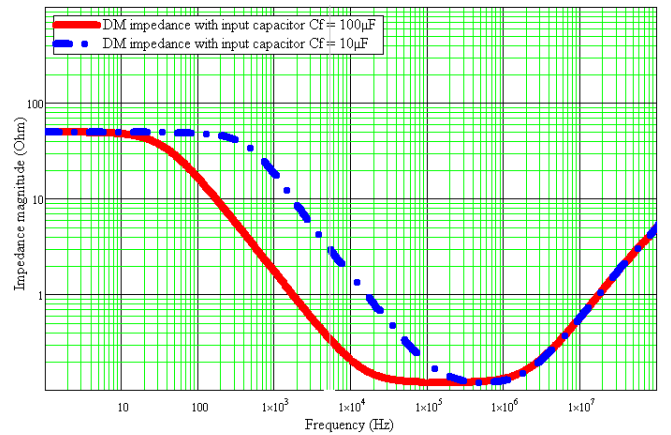
Fig. 17. The comparison between two DM impedances profile about two values of the input capacitors C_f = \{10\mu F, 100\mu F\} .
