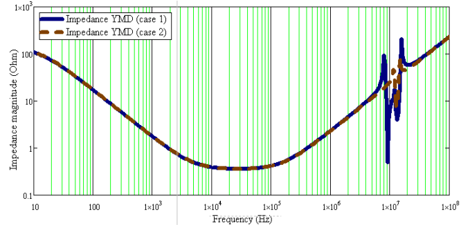
Fig. 20. Y_{MD} impedance for two capacitances value of the Mosfet
