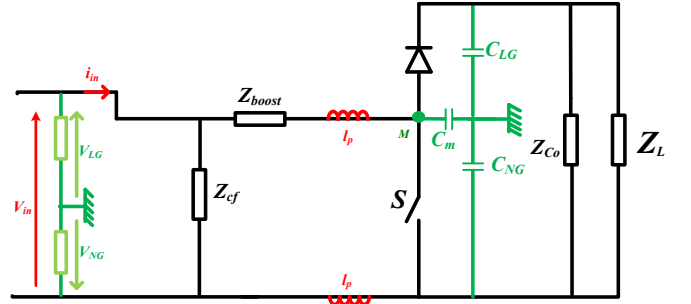
Fig. 9. The boost converter under study.
