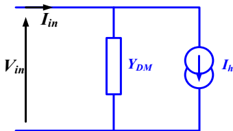
Fig. 7. Converter's models.
