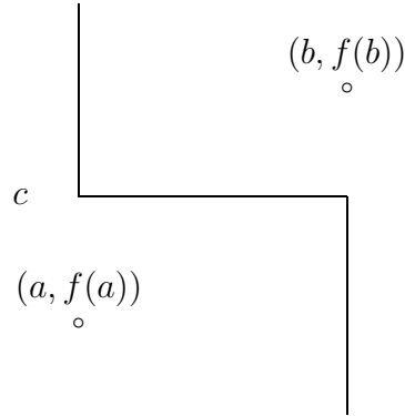
Figure 1: h -shape set H
