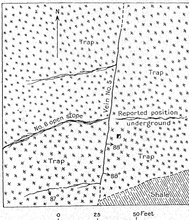
FIGURE 13.—Sketch showing position of principal veins in Lubec lead mine.
