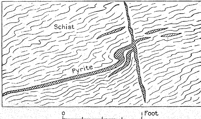
FIGURE 3.—Quartz-pyrite veinlet leading off from Twin Lead lode. The crumpling of the pyrite shows that it is older than the metamorphism of the inclosing Ellsworth schist.
