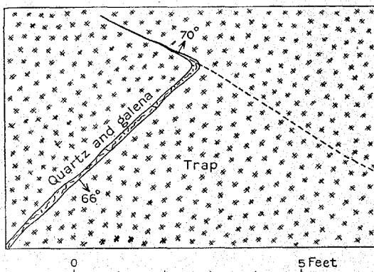
FIGURE 14.—Small vein in Lubeck lead mine. The vein is later than the fissure in which it ends.
