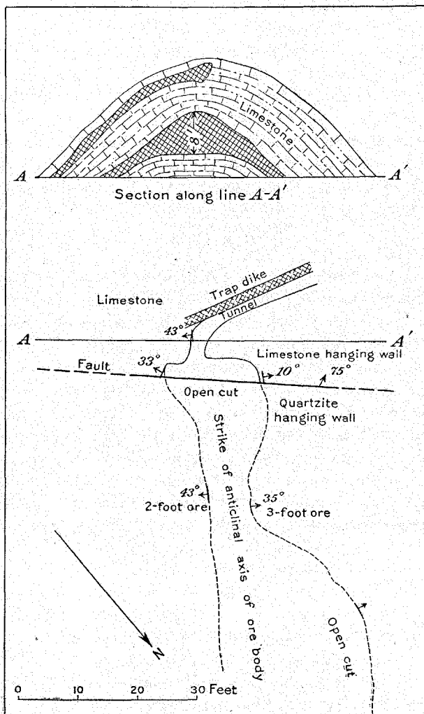
FIGURE 16.—Plan and cross section of the Robinson mine, near Concord, Somerset County.
