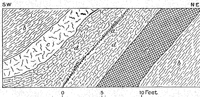
FIGURE 21.—Section of vein at east end of 115-foot level, 40 feet above floor, Milan mine. a , Oxidized streak; b , schist; c , massive quartz, pyrite, and galena; d , pyritiferous schist or milling ore; e , massive pyrite.
