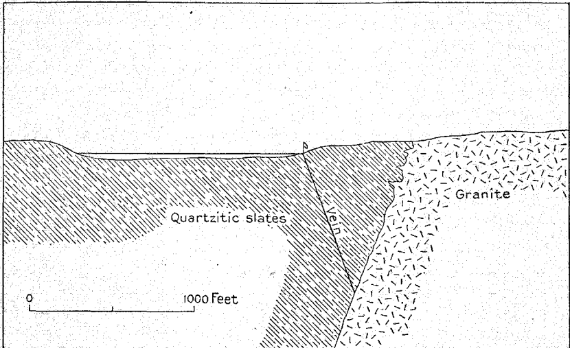
FIGURE 12.—Cross section of the Sullivan mine. (After Kempton.)
