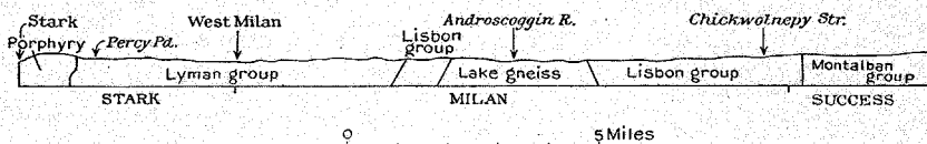
FIGURE 19.—Geologic east-west cross section through West Milan, N. H., north of the Milan copper mine. (After Hitchcock, Atlas of New Hampshire, 1878.)
