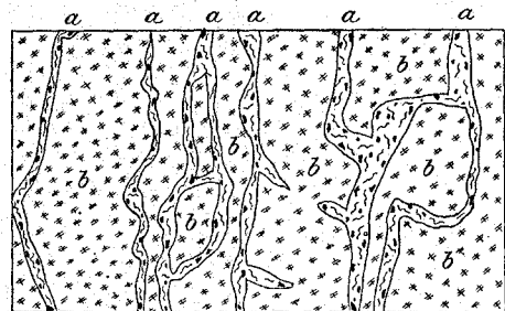
FIGURE 9.—Brecciated diabase cut by quartz and sulphides, Pembroke mine. a , Quartz and ore; b , diabase.
