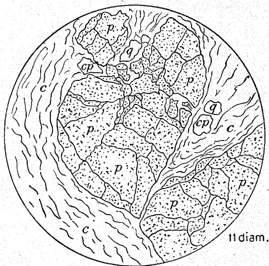
FIGURE 6.—Thin section of ore from Milan mine, New Hampshire. The pyrite has been shattered and recemented. p , Pyrite; cp , chalcopyrite; c , chlorite; q , quartz.
