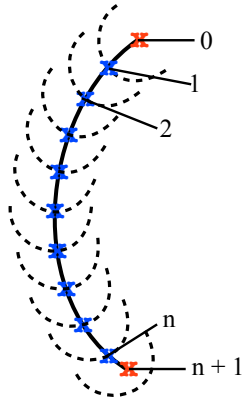
Figure 1. Schematic diagram of the separator tracing algorithm.
