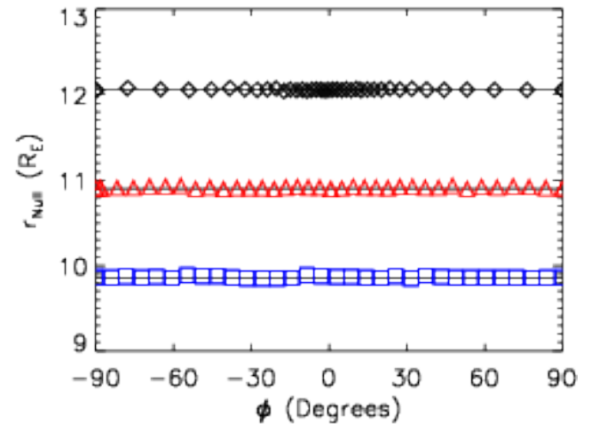
Figure 3. Verification of the separator tracing algorithm for \theta_{\text{IMF}} = 30^\circ (black diamonds), 90^\circ (red triangles), and 150^\circ (blue squares) using vacuum superposition. The exact solutions for the separator are shown as solid (black) lines.
