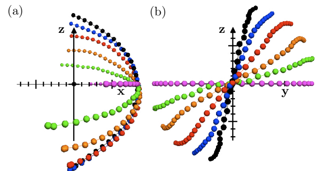
Figure 8. Plot of separators in global MHD simulations for \theta_{\text{IMF}} = 30^\circ (black), 60^\circ (blue), 90^\circ (red), 120^\circ (orange), 150^\circ (green), 180^\circ (purple) looking (a) duskward and (b) earthward.
