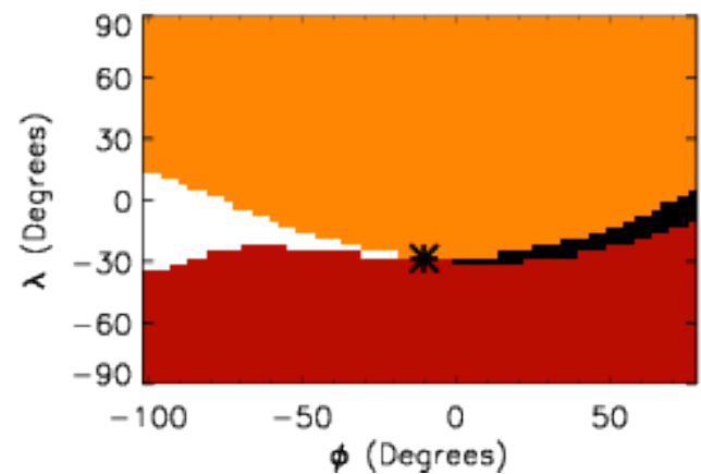
Figure 2. Sample topology map for \theta_{IMF} = 30^\circ for a hemisphere centered at \mathbf{r} = (3.16, 1.87, 8.01) R_E , with radius of 1 R_E . Colors denote magnetic topology: red are closed terrestrial fields, orange are open solar wind fields, black and white are half-closed fields that terminate at the south and north poles of Earth, respectively. The black asterisk marks the approximate separator location.
