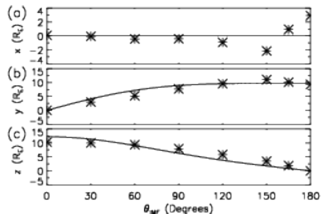
Figure 6. Plots of magnetic null (a) x -coordinate, (b) y -coordinate, and (c) z -coordinate as a function of IMF clock angle \theta_{\text{IMF}} . Solid lines display vacuum superposition prediction from Eqs. (8)–(10) and asterisks are the coordinates of nulls in the MHD simulations.
