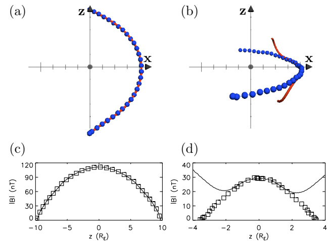
Figure 7. Comparison between traced separators and the last closed field line in global MHD simulations. The last closed field line is a solid (red) line and the determined separator locations are (blue) spheres for \theta_{\text{IMF}} of (a) 30^\circ and (b) 150^\circ . The magnetic field strength |\mathbf{B}| as a function of z -coordinate along the separator is a solid line for the last closed field line and as squares for the traced separator for \theta_{\text{IMF}} (c) 30^\circ and (d) 150^\circ .
