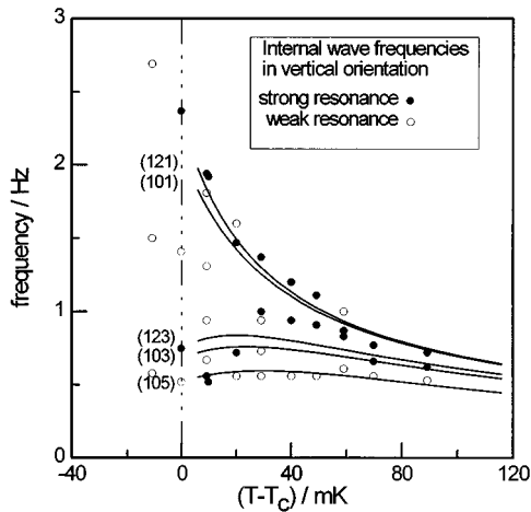
FIG. 10. Internal wave frequencies measured (circles) and calculated (lines) with the cell's axis held vertical. As many as five modes could be seen at one temperature, consistent with the greater number of modes allowed by symmetry than for the horizontal orientation. "Strong" and "weak" indicate the excited mode's observed amplitude.
