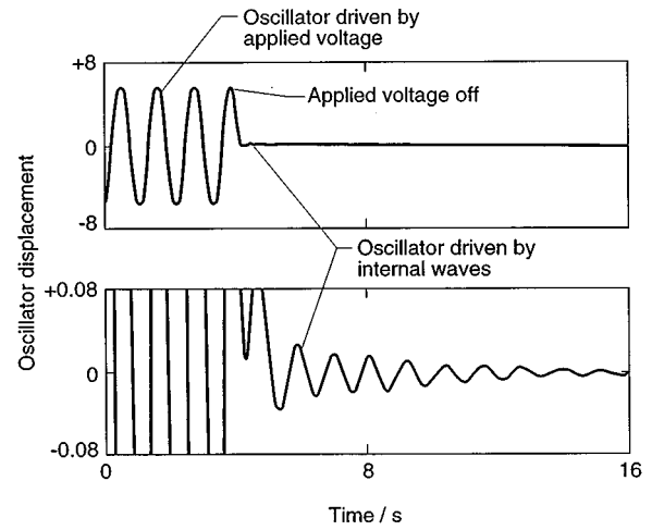
FIG. 4. Example of an internal wave frequency measurement. (a) The oscillator's displacement shown during and after application of an oscillating torque at 0.875 Hz. (b) The oscillator's displacement during the same interval, magnified by 100.
