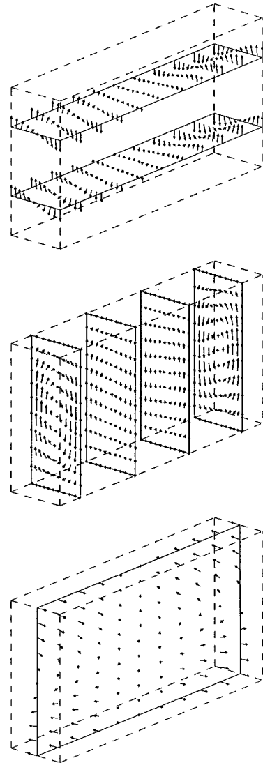
FIG. 6. The flow field of mode (111) calculated by Eqs. (9) and (11) for the special case of an exponential profile with N^2 = 25 \text{ s}^{-2} . The coordinates correspond to those of Figure 3b. In the lowest view, the arrows were lengthened by a factor of 2 relative to those in the upper two views.
