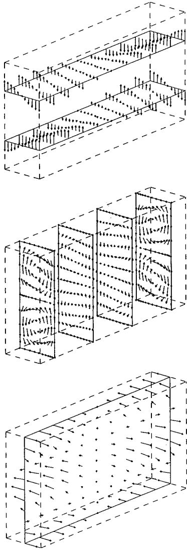
FIG. 7. The flow field of mode (112) calculated by Eqs. (9) and (11) for the special case of an exponential profile with N^2=25 \text{ s}^{-2} . The coordinates correspond to those of Figure 3b. In the lowest view, the arrows were lengthened by a factor of 2 relative to those in the upper two views.
