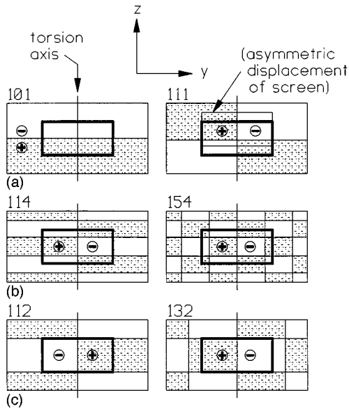
FIG. 8. Symmetry and geometry determined which internal wave modes coupled to the oscillating screen. The cell is in the horizontal orientation and the screen's location in the yz plane is indicated by the rectangular outline. (a) Examples of modes whose symmetry did not allow coupling to oscillating screen. [A slight vertical displacement of the oscillator allowed coupling to mode (111).] (b) Examples of modes allowed by symmetry but discouraged by geometrical cancellation of torques on the screen. (c) Examples of modes allowed by both symmetry and geometry.
