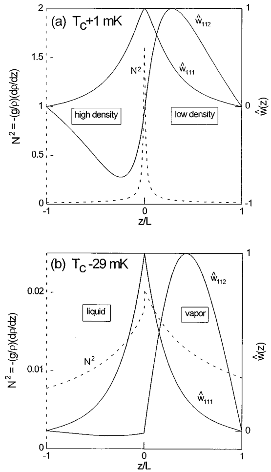
FIG. 9. Plots of the squared Brunt-Väisälä frequency N^2 and the vertical component of the velocity \hat{w} calculated as a function of the normalized height. (a) At T_c + 1 mK, mode (111) is nearly symmetric and strongly samples the steep density gradient near the cell's midplane. In contrast, mode (112) has little vertical velocity near the midplane. (b) At T_c - 29 mK, mode (112) is confined almost entirely to the upper, vapor half of the cell, and thus its frequency is determined chiefly by the average value of N^2 in that region.
