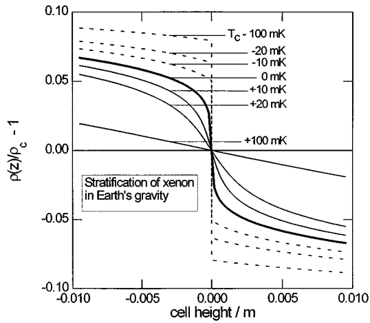
FIG. 1. The density profile of the xenon sample calculated by Eqs. (1) at various reduced temperatures. Far above T_c , the height dependence is weak and approximately linear. At T_c , the density gradient is infinite at the middle height, where \rho = \rho_c . Far below T_c , the xenon separates into liquid and vapor layers, each of nearly constant density.
