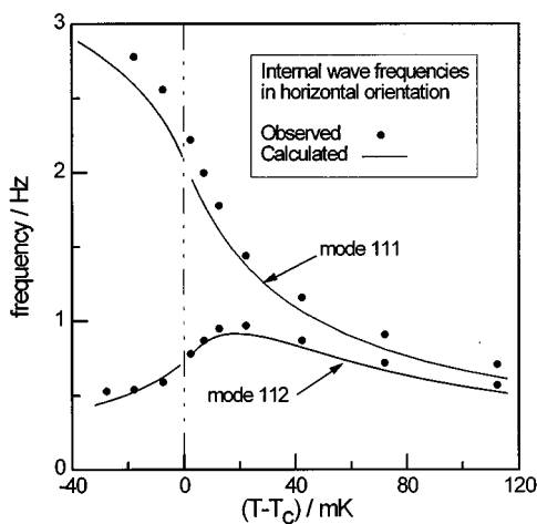
FIG. 2. Internal wave frequencies, measured (circles) and calculated (lines). The cell's axis was horizontal and the screen's torsion axis was vertical, so that the screen's motion was horizontal. The numerical calculations used the actual profiles derived from xenon's equation of state.
