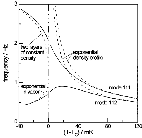
FIG. 5. Comparison between numerically (solid lines) and analytically (dashed lines) computed internal wave frequencies for the horizontal orientation. Above T_c + 60 mK, the linear density profile can be approximated by an exponential, allowing use of Eq. (10), which matches the numerical results. Below T_c , the fluid is separated by an interface into liquid and vapor layers. Neglect of the stratification within each layer allows use of Eq. (20), which describes mode (111)'s temperature dependence at temperatures below T_c - 5 mK. Neglect of the liquid layer entirely and assumption of an exponential density profile within the vapor phase allows the use of Eq. (10) to approximate the temperature dependence of mode (112) below T_c - 5 mK.
