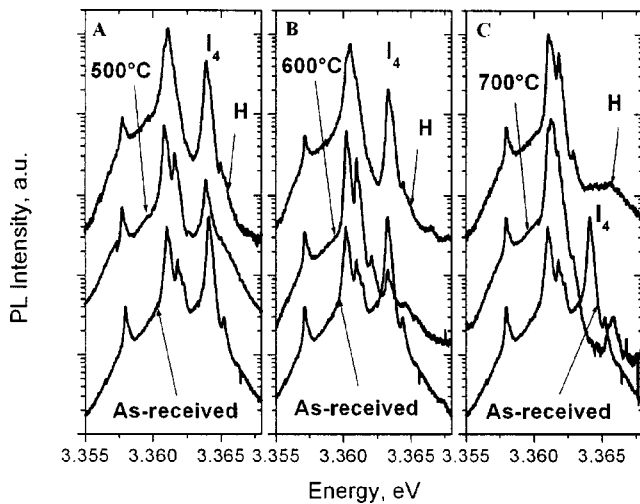
FIG. 1. PL results for the air-annealed CVT samples in the near band edge region, T=10 K, incident power= 0.2 W/cm 2 . The BEx peaks shown for the as-received CVT material are commonly observed. (A) After anneal in air for 30 min at 500 °C, the relative intensity of the I_4 line ( E=3.363 eV) is reduced. 1 h of remote H-plasma treatment partially restores the intensity of I_4 . (B) After anneal in air for 30 min at 600 °C, the I_4 line is not discernible. 2 h of hydrogenation bring back the I_4 . (C) After anneal in air for 30 min at 700 °C, the I_4 line is not discernible, 3 h of hydrogenation restore a small shoulder around 3.363 eV.
