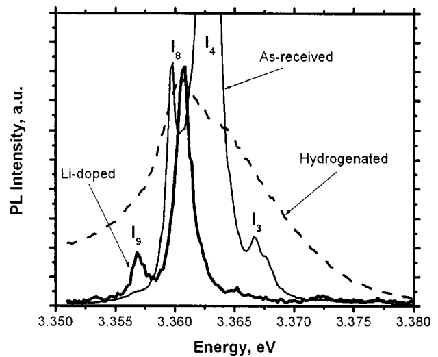
FIG. 2. PL results for the Li-doped CVT sample in the near band edge region, T=10 K, incident power= 0.2 W/cm 2 . After Li-diffusion treatment, the I_4 line is suppressed. Subsequent H-plasma treatment broadens the bound-exciton emission and restores a shoulder at \sim 3.364 eV.
