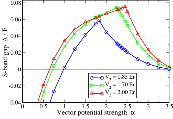
FIG. 18: (Color online) The s band gap as function of the vector potential strength for several values of the super-lattice generating component V_2 . The main amplitude of the optical lattice potential is fixed, V_1 = 3.4E_r . Notice that each curve has a singularity point and that the slope to the left (right) of the singularity point is positive (negative). The positive slope correspond to an indirect gap between the maximum of the lower band at (\pi, \pi) and the minima of the upper band at (0, \pi)/(\pi, 0) , while the negative slope corresponds to a direct gap at \pi, \pi . Note that for weak vector potentials with the strength \alpha below a critical value \alpha^*(V_2) the indirect gap becomes negative.
