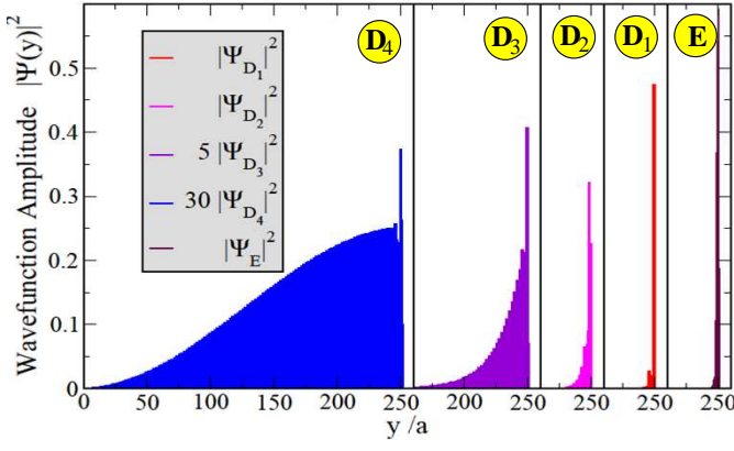
FIG. 10: (Color online) Spatial dependence of the “amplitude” function |\Psi_{k_x, y}|^2 = \sum_{(n,m)} |\widetilde{\Psi}_{k_x, y}^{(n,m)}(y_j)|^2 for state E and for the sequence of states D_1 \rightarrow D_4 from Fig. 8. D_1 is positioned in the middle of the gap, while D_4 is at the gap edge and has bulk character. During this transition the characteristic length scale for the exponential decay of the edge states increases continuously from a value of a few lattice sites to a value comparable to the width of the stripe. The state E has a very pronounced edge character, but is not topologically protected. Note that the horizontal axis was translated for clarity.
