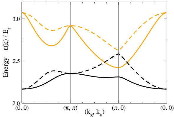
FIG. 5: (Color online) Energy dispersion for the first two bands of the square super-lattice model along the (0,0) \rightarrow (\pi, \pi) \rightarrow (\pi, 0) \rightarrow (0,0) path in the Brillouin zone. The full lines correspond to the parameters from Fig. 4(c). The dashed lines show the energy dispersion obtained if we neglect the hybridization with higher-energy bands.
