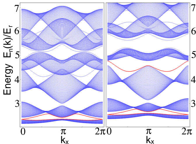
FIG. 17: (Color online) The band structure of the Hamiltonian given by Eq. (3) in the stripe geometry. The left panel corresponds to the parameters V_1 = 3.4E_r , V_2 = 1.7E_r and \alpha = 2\hbar/a , while the right panel corresponds to a slightly deeper lattice with V_1 = 3.7E_r . Note that there are no edge states between the second and the third bands, but an edge mode is clearly visible between the third and the fourth bands. Increasing V_1 opens a gap in the spectrum (right panel) and reveals the topological nature of that edge mode. By contrast, the edge states that populate the gap between the fourth and the fifth bands are topologically trivial, as they do not connect the two bands.
