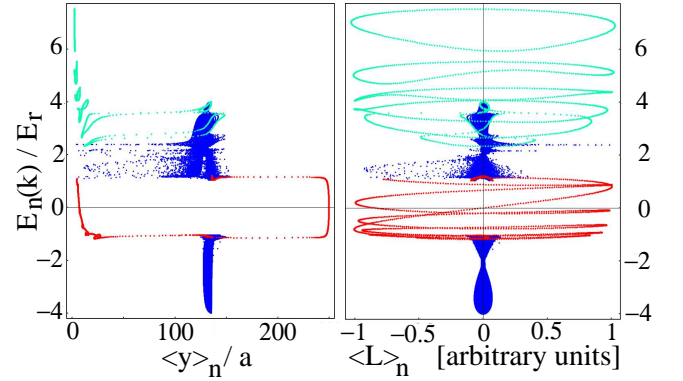
FIG. 31: (Color online) Average position (left panel) and average angular momentum (right pane) for a stripe with a soft boundary and same parameters as in Fig. 28.
