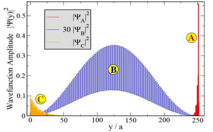
FIG. 9: (Color online) Spatial dependence of the “amplitude” function |\Psi_{k_x, \nu}|^2 = \sum_{(n,m)} |\tilde{\Psi}_{k_x, \nu}^{(n,m)}(y_j)|^2 for the states marked by the letters A, B and C in Fig. 7. The stripe has a width d = 252 (in units of a = 1/\sqrt{2} ). State A, which is well inside the bulk gap, is localized near the upper edge and decays exponentially with a characteristic length scale of a few lattice constants. State B, which is at the gap edge, is a bulk state with a smoothly varying envelope function. Notice the multiplication factor of 30 introduced to make the function visible on the same scale as the edge states. State C belongs to the edge mode but is very close to the gap edge. It is localized near the bottom edge and decays exponentially but has a length scale significantly larger than state A.
