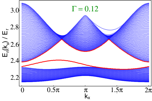
FIG. 20: (Color online) Band structure for a stripe with inequivalent edges and with the same parameters as in Fig. 19. For \Gamma = 0.12E_r the system is a standard band insulator but, in contrast with the equivalent edge case (see Fig. 19), a well-defined edge mode populates the gap. A clean insulator with the chemical potential inside the bulk gap supports gapless edge excitations. However, any small perturbation (such as disorder or interactions) will open a gap in the edge mode.
