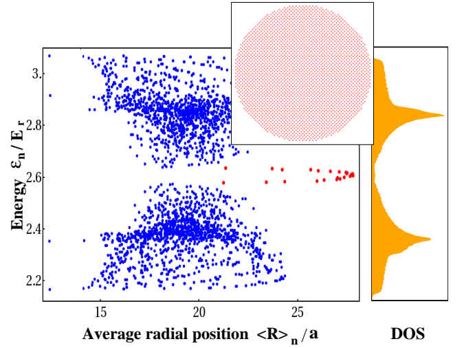
FIG. 14: (Color online) Diagram showing the average radial position versus energy for the single-particle states of a system described by Eq. (3) in a confining potential (12). The parameters of the system are V_1 = 3.4E_r , V_2 = 1.7E_r , and \alpha = 2\hbar/a . The underlying lattice (i.e., the minima of the effective optical lattice potential) is shown in the inset. The edge states are characterized by values of \langle r \rangle_n comparable with R_0 = 29a , the disk radius, as a result of their localization in the vicinity of the boundary. The clearly defined edge mode crosses the bulk gap and connects the lower and upper bands, thus revealing its topological nature. The density of states (right) is practically identical with that shown in Fig. 13(a) for a similar system with stripe geometry.
