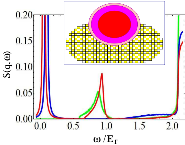
FIG. 34: (Color online) Dynamical structure factor for a system described by Eq. (1) with t_1 = (1 + 0.3i)E_r , t_2 = -0.3E_r and t'_2 = 0.3E_r . The blue (dark gray) line corresponds to a sharp boundary, while the red (gray) line is for a soft boundary with the same profile as in Fig. 28. The extra in-gap contribution represents transitions between different branches of the soft edge mode. The green (light gray) line corresponds to the same parameters as the red curve and opposite scattering wave vector -\mathbf{q} . Note the absence of the low-energy peak. The inset is a schematic illustration of the intersecting laser beams illuminating a portion of the system.
