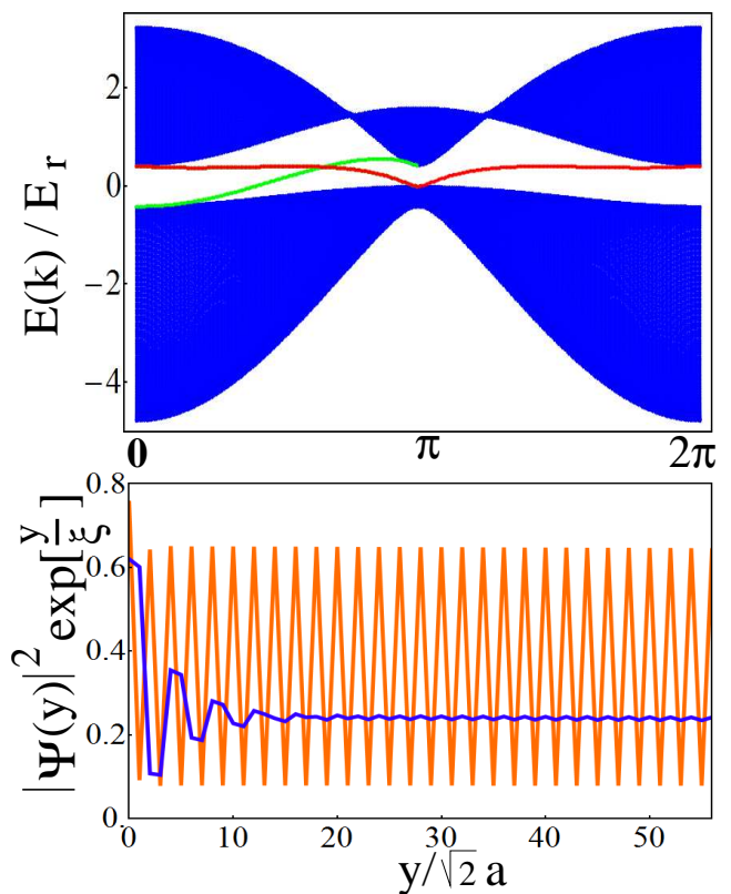
FIG. 23: (Color online) (Upper panel) Spectrum for the square superlattice model (1) with parameters t_1 = (1 + 0.2i)E_r , t_2 = -0.3E_r , and t'_2 = -0.06E_r in the stripe geometry. The system is finite in the y direction and infinite in the x direction, with the axes are oriented along the next-nearest neighbor directions (see Fig. 3). For an odd number of layers (i.e., equivalent edges) the edge states (red/dark gray lines) with k_x < \pi are localized near y = 0 , while the edge states with k_x > \pi are localized near the opposite boundary. For an even number of layers (i.e., inequivalent edges) the mode localized near y = 0 remains unchanged, while the other mode is now characterized by k_x < \pi (green/light gray line). (Lower panel) Edge state amplitudes multiplied by exponential factors to reveal the oscillatory behavior. Blue (dark gray): edge state corresponding to k_x = 0.97\pi/\sqrt{2}a and \xi = 1.441\sqrt{2}a . Orange (light gray): edge state with k_x = 0.7\pi/\sqrt{2}a and \xi = 1.351\sqrt{2}a .
