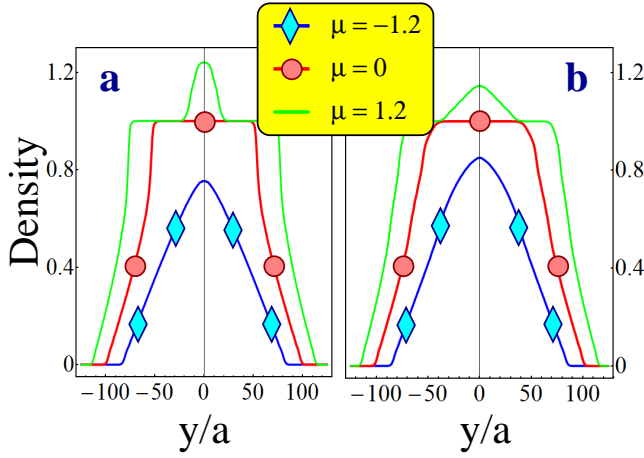
FIG. 33: (Color online) Density profiles for a fermionic system with harmonic confinement and different values of the chemical potential. Panel (a) corresponds to a topological insulator model, while panel (b) shows the density of a standard insulator. The parameters for the models are the same as in Fig. 32. Note the plateaus characterized by \rho = 1 (particles per lattice site), which correspond to the insulating phase. No qualitative difference can be observed between the two types of models.
