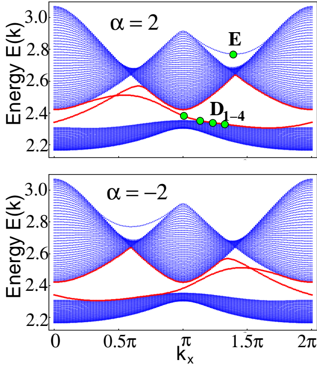
FIG. 8: (Color online) Band structure for a stripe with inequivalent edges (see main text). All the sites on one boundary belong to the A sublattice, while all the sites on the other boundary are B -type. For the top panel the parameters are the same as in Fig. 7, the only difference being an extra line of lattice sites at one of the boundaries. Notice the completely different dispersion of the edge modes and the different location of the degeneracy point. The symmetry between left-moving and right-moving states is broken. A mirror image of the dispersion lines can be obtained by adding the extra line of lattice sites to the opposite edge, or by reversing the direction of the vector potential, \alpha \rightarrow -\alpha (lower panel). A topologically trivial edge mode develops at the top of the second band (state E belongs to this mode).
