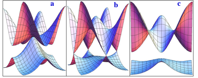
FIG. 4: (Color online) Spectrum of the square super-lattice model with periodic boundary conditions (no boundaries). Only the lowest two bands are shown, although four other bands were considered in the calculation. The wave-vector takes values in the first Brillouin zone, 0 \leq k_x \leq 2\pi/\sqrt{2}a , 0 \leq k_y \leq 2\pi/\sqrt{2}a , and we make the choice of length units a = 1/\sqrt{2} . (a) If V_2 = 0 (no super-lattice structure), the two bands are degenerate at \mathbf{k} = (\pi, \pi) . (b) If \alpha = 0 (no vector potential), the gap closes at two Dirac points (0, \pi) and (\pi, 0) . (c) For V_1 = 3.4E_r , V_2 = 1.7E_r and \alpha = 2\hbar/a a full gap opens. The bands are shown along the k_x direction (with k_y out of the plane).
