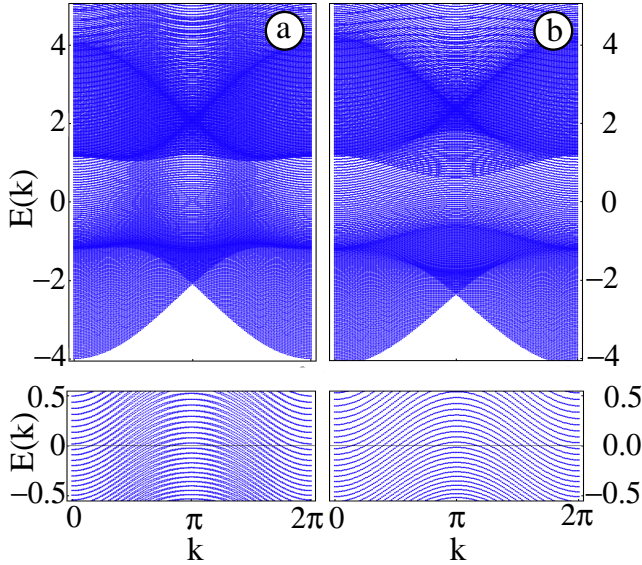
FIG. 32: (Color online) Spectrum of a system with harmonic confining potential. Panel (a) corresponds to a square superlattice topological “insulator” model with the same parameters as in Fig 28, while panel (b) represents a standard insulator model on the square superlattice with t_1 = E_r , t_2 = -0.3E_r , t'_2 = 0.3E_r and a staggered on-site potential \pm\Gamma with \Gamma = E_r . The lower panels show the low energy spectra that characterize the inhomogeneous topological (left) and normal (right) metals. Note that the topological metal has a spectrum consisting of two modes that are qualitatively the same as the soft mode shown in Fig. 29 (in the present case both boundaries are soft). By contrast, the spectrum of the normal metal contains many disconnected modes.
