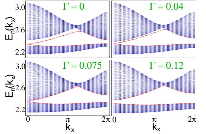
FIG. 19: (Color online) Band structure for a system with stripe geometry described by the parameters V_1 = 3.4E_r , V_2 = 1.7E_r , \alpha = 2\hbar/a and different values of the staggered potential \Gamma (given in units of E_r ). \Gamma = 0 corresponds to the case shown in Fig. 7. Applying a small staggered potential reduces the gap in the vicinity of k_x = 0 (top right panel). At the critical value \Gamma_c \approx 0.075E_r , the gap closes at k_x = 0 , while for \Gamma > \Gamma_c a full gap opens again. At large values of \Gamma the system is a standard band insulator with no edge modes inside the gap. Notice that the spectra are shown for half of the one-dimensional Brillouin zone while the other half can be obtained by mirror symmetry with respect to k_x = \pi .
