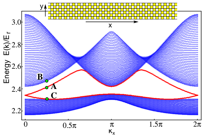
FIG. 7: (Color online) The band structure of Eq (3) in the stripe geometry. The corresponding lattice is schematically shown in the inset. Notice the edge state modes that populate the gap and merge with the bulk states. The edge modes cross the gap connecting the lower and upper bands and intersect at k_x = 0 due to Kramers degeneracy. Small perturbations can modify the dispersion of the edge modes and the location of the Kramers degeneracy points, but cannot open a gap for the edge states. Notice that the bulk bands can be obtained by projecting the two-dimensional spectrum shown in Fig. 4(c) on a plane perpendicular to the y axis. The same set of parameters as in Fig. 4(c) was used.
