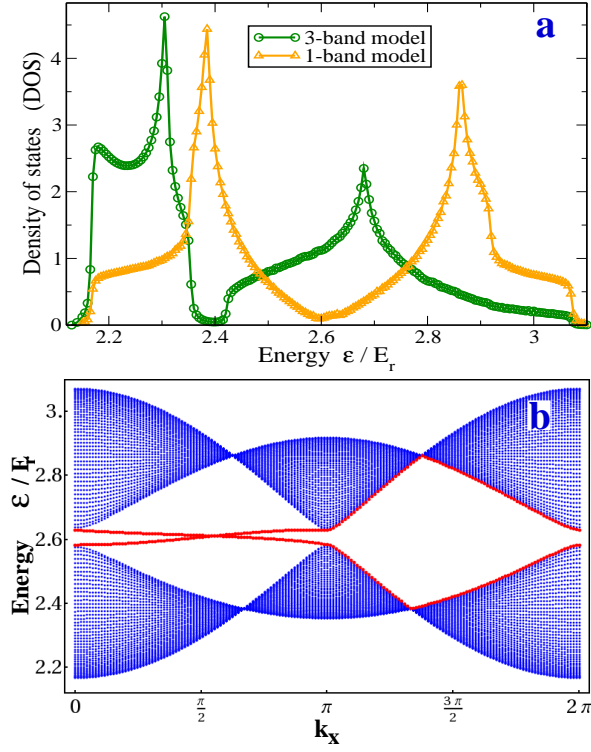
FIG. 13: (Color online) Density of states (a) and spectrum (b) showing the s bands of a stripe with inequivalent edges calculated within a simplified tight-binding approximation that neglects hybridization with higher bands. For comparison, the density of states calculated within a three-orbital tight-binding approximation is also shown. The corresponding spectrum is given in Fig. 8 (top panel). Note that the topology of the edge modes is not altered, in spite of a significant redistribution in the density of states.
