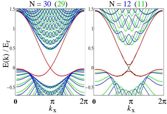
FIG. 25: (Color online) Opening of a gap in the edge state spectrum due to finite size effects. The system is a thin stripe with the same geometry and hopping parameters as in Fig. 24. The size of the gap is determined by the overlap of edge states localized on opposite boundaries and, consequently, varies roughly exponentially with the width of the stripe and inherits the oscillatory behavior of the edge states. For large N the edge states are gapless and independent of parity. For thin films, a finite gap opens in systems with even number of layers, while systems with odd number of layers remain gapless. Note that the “bulk” spectrum varies dramatically with the system size, in contrast with the edge modes that are practically unaffected if the system size is much larger than their characteristic length scale.
