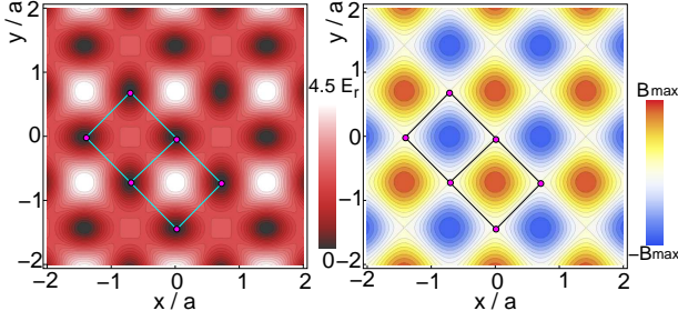
FIG. 3: (Color online) (Left) Optical super-lattice potential corresponding to V_1 = 3.4E_r , V_2 = 1.7E_r and \alpha = 2\hbar/a (see main text). A unit cell consisting of two squares with side length a is marked with light blue (light gray) lines. Notice the \pi/2 rotation of the axes relative to lattice in Fig. 2(b). (Right) Effective "magnetic" field generated by the vector potential \mathbf{A}(\mathbf{r}) . The total flux through the unit cell is zero.
