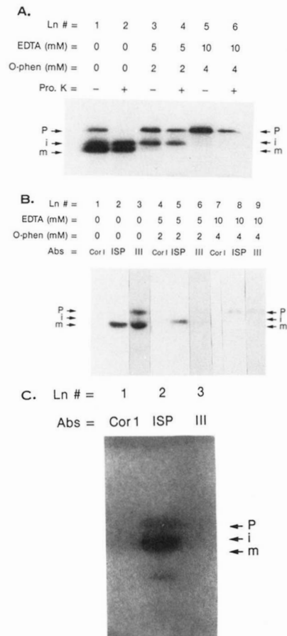
FIG. 2. Effect of inhibitors on import and assembly of the iron-sulfur protein into the cytochrome bc_1 complex. A , the import of the ^{35}\text{S} -labeled precursor form of the iron-sulfur protein into mitochondria isolated from the wild-type yeast strain 777-3A was performed in the presence of inhibitors as described under "Experimental Procedures." B , After the import reaction in the presence of 5 mM EDTA and 2 mM o -phenanthroline (lanes 4–6) or 10 mM EDTA and 4 mM o -phenanthroline (lanes 7–9), mitochondria were solubilized with 1% Triton X-100, then immunoprecipitated by specific antisera as indicated, and analyzed by SDS-PAGE and fluorography. C , experimental conditions were identical with those of panel B , except that the import reaction occurred in the presence of 5 mM EDTA and 2 mM o -phenanthroline, and mitochondria were treated with 3% SDS prior to immunoprecipitation with specific antisera as indicated. O-phen , O -phenanthroline. Other abbreviations are as defined in the legend to Fig. 1.
