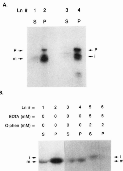
FIG. 3. Localization of imported forms of the iron-sulfur protein in the mitochondrial membranes after sonication. Import of the ^{35}\text{S} -labeled iron-sulfur protein into isolated mitochondria of the wild-type strain 777-3A in the absence (lanes 1 and 2) and presence (lanes 3 and 4) of 5 mM EDTA and 2 mM o -phenanthroline was performed as described under "Experimental Procedures." After the import reaction, mitochondria were reisolated and resuspended in 0.6 M sorbitol and 20 mM Hepes/KOH (pH 7.4) and sonicated as indicated under "Experimental Procedures." The sonicated mixture was separated into pellet and supernatant fractions by centrifugation at 100,000 \times g for 1 h. Both pellet and supernatant portions were divided into two equal portions. A , one half of both pellet and supernatant was directly analyzed by SDS-PAGE and fluorography. B , the remaining half of the pellet was solubilized with 1% Triton X-100, and then both pellet and supernatant were immunoprecipitated with antisera against either the iron-sulfur protein (lanes 1 and 2) or the bc_1 complex (lanes 3–6), as described under "Experimental Procedures." The immunoprecipitates were analyzed by SDS-PAGE and fluorography. S, supernatant, and P, pellet. Other abbreviations are as defined in the legends to Figs. 1 and 2.
