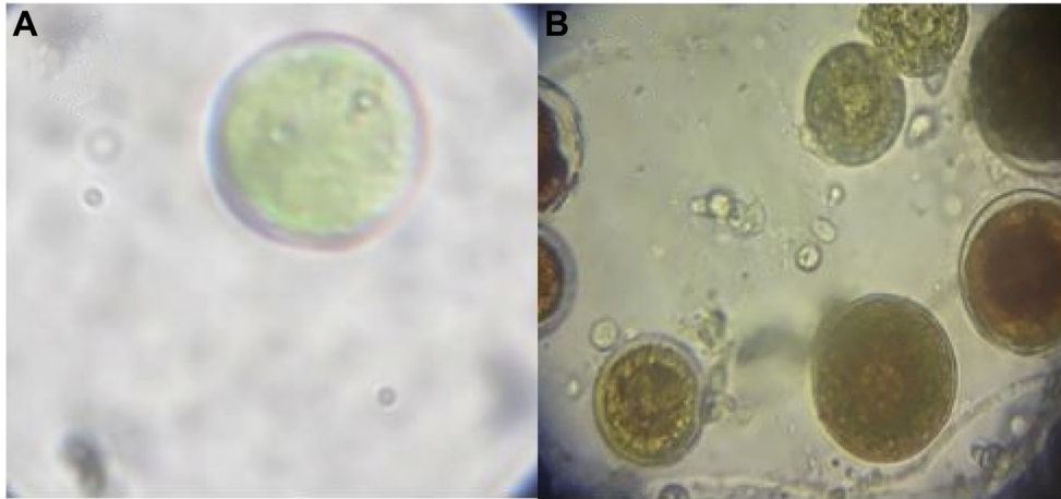
Figure 3. Microscopic images of Haematococcus pluvialis at (A) day 0 and (B) day 22.
