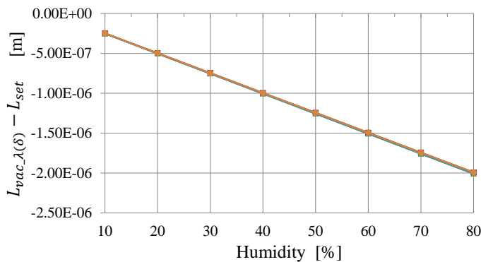
FIG. 6 Change in L_{vac,\lambda} and L_{vac,\delta} with respect to changes in the barometric pressure and humidity. Note that all lines overlap when P \in [80, 120] kPa.
