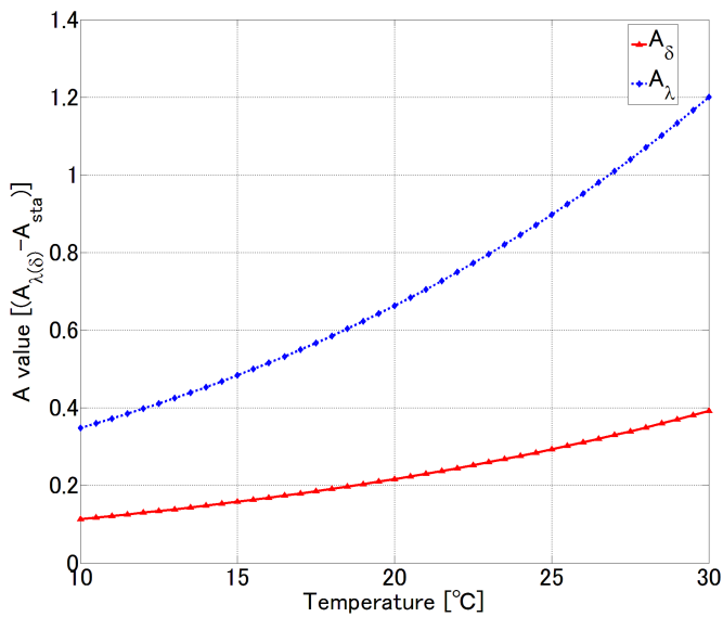
FIG. 1 Change in the A_\lambda and A_\delta factors of the refractive indices with respect to changes in the temperature (humidity = 50%).
