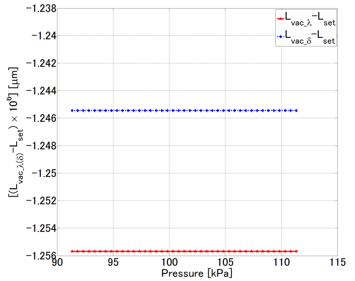
FIG. 4 Change in L_{vac,\lambda} and L_{vac,\delta} with respect to changes in the barometric pressure (humidity = 50%).
