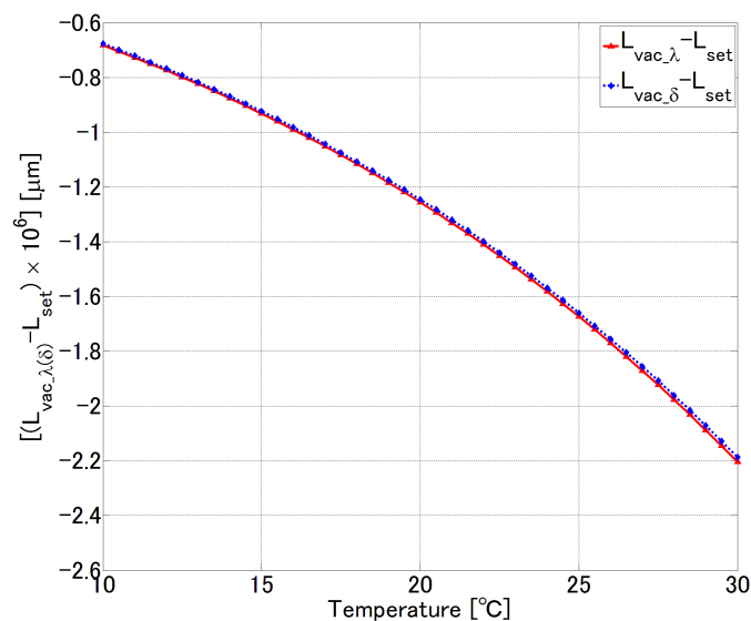
FIG. 3 Change in L_{vac,\lambda} and L_{vac,\delta} with respect to changes in the temperature (humidity = 50%).
