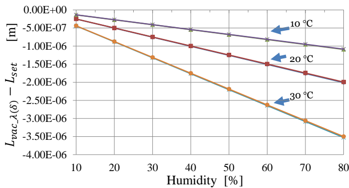
FIG. 5 Change in L_{vac,\lambda} and L_{vac,\delta} with respect to changes in the temperature and humidity. The lines showing the difference between L_{vac,\lambda} and L_{vac,\delta} overlap each other when T = 10^\circ\text{C} , 20^\circ\text{C} and 30^\circ\text{C} , respectively.
