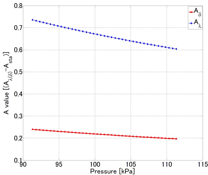
FIG. 2 Change in the A_\lambda and A_\delta factors of the refractive indices with respect to changes in the barometric pressure (humidity = 50%).
