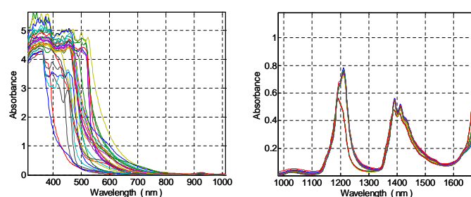
FIG. 2 Absorption spectra of the entire collection of lubricant oils in the UV-VIS (left) and NIR (right) spectral bands.
