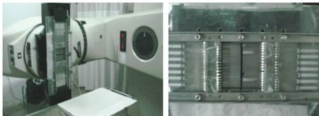
Figure 1: Prototype 1 MLC configured in ROPS TPS (reprinted with permission from Ayyangar et al. 10 )
