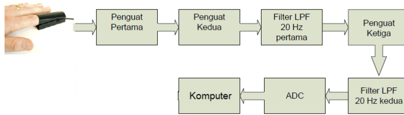
Gambar 6. Block Diagram Umum Photoplethysmograph
