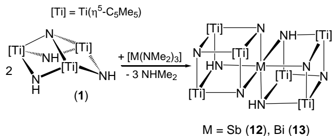
Scheme 4. Reactions of 1 with [\text{M}(\text{NR}_2)_3] group 15 derivatives.
