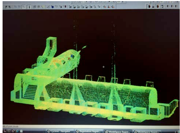
Figure 10. Three-dimensional model of the vault complex. The model was built by composing the sets of data collected with the scanner laser along the field work. Upper and lower main spaces can be clearly seen, as well as the inner stair and the wall-embedded access stair.
