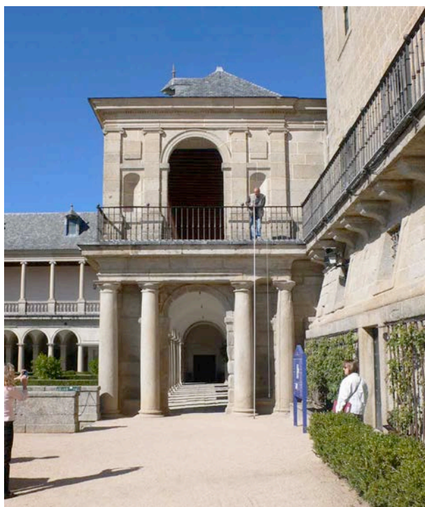
Figure 6. Differences of height between the external station points were directly measured with tape and plumb. Increases lately added were taken into account, as well as the difficulties introduced of the sloped wall of the Monastery's south façade.
