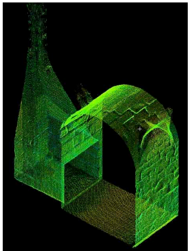
Figure 11. Detail of a smokestack and a section of the vault in the lower cellar.
