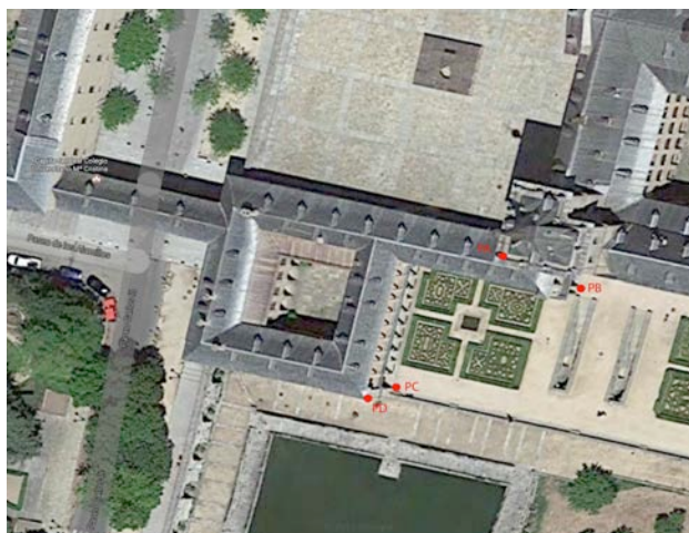
Figure 7. Location of the external control points.
