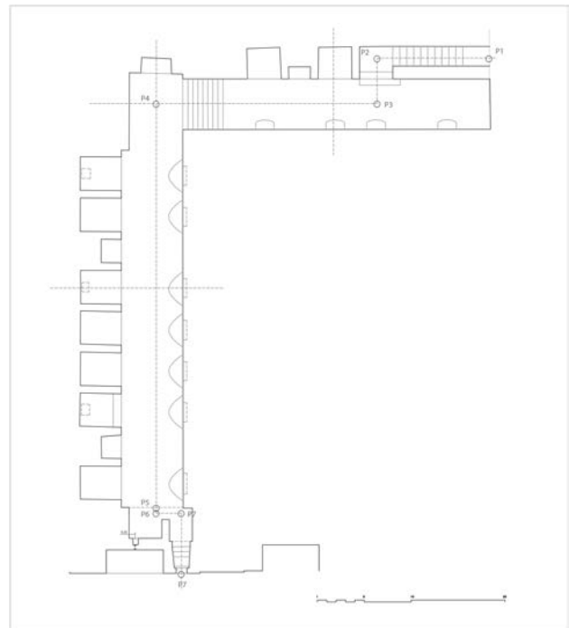
Figure 5. Control points in the cellars used in the traversing method.
