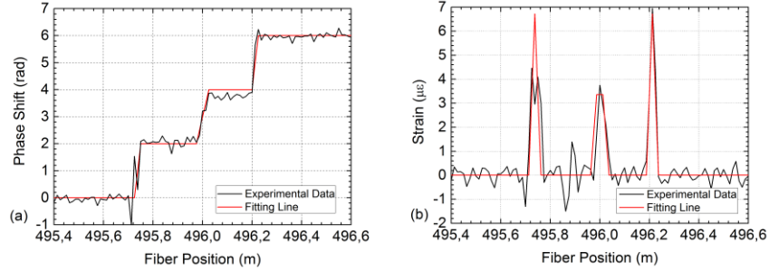
Fig. 4. (a) Phase variation of the \Phi OTDR signal along the fiber when strain is applied in three fiber sections 1,2,3 of length 2.5cm/5cm/2.5cm by a translation stage. (b) Correspondent calculated strain variation along the fiber.
