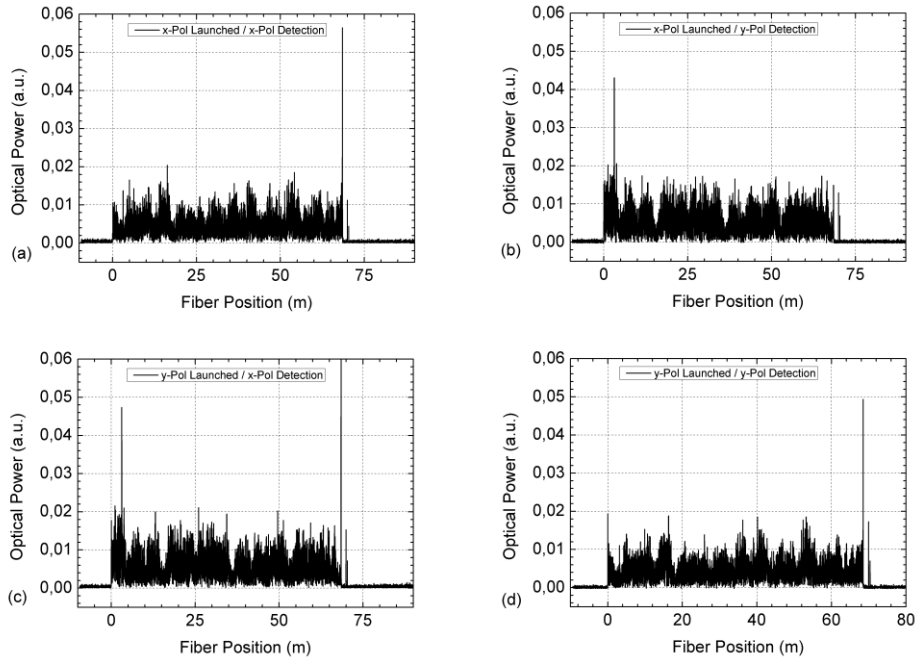
Fig. 6. Optical Power of the \Phi OTDR decoded signal along the fiber launching dual polarization QPSK data. Figures show the impulse response of the fiber when data is sent on the x polarization and detected on the (a) x polarization (b) y polarization; data is sent on the y polarization and detected on the (c) x polarization (d) y polarization.
