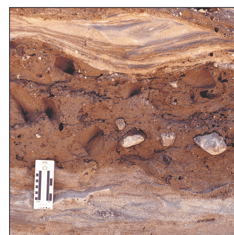
Sand with interbedded flowfill: s-ds(tf) -- Close-up of pit face in an end-moraine, Westbrook, showing part of a stony flowfill lens (center) deposited where a glacier margin terminated in the sea.
