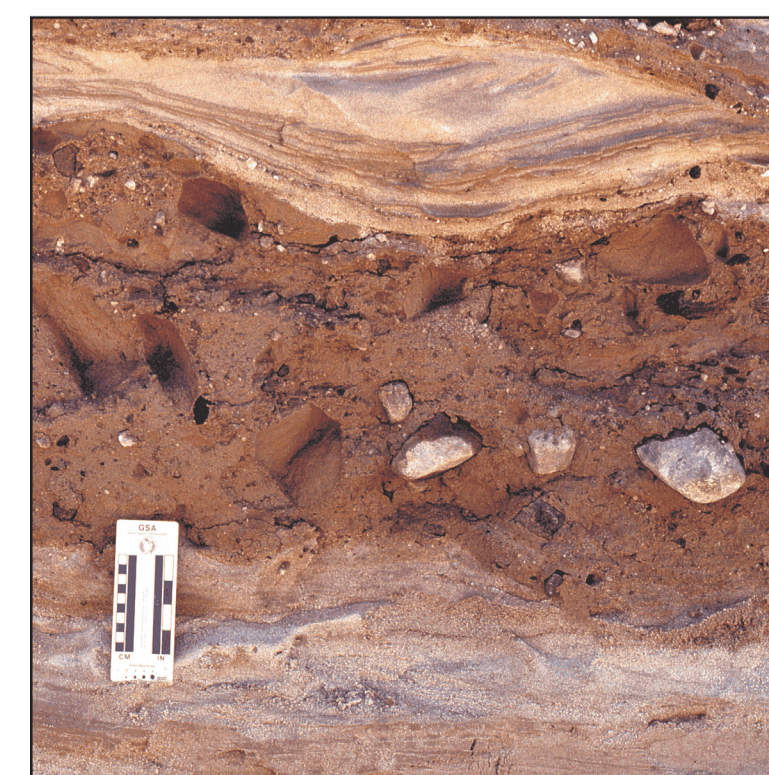
Sand with interbedded flowfill: s±ds(tf) -- Close-up of pit face in end-moraine, Westbrook, showing part of a stony flowfill lens (center) deposited where glacier margin terminated in the sea.
