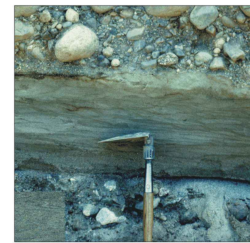
Gravel over sand over gravel: p-c/s/p-c -- Close-up of pit face showing interbedded sand unit between pebble-cobble gravel beds in upper part of glaciomarine delta, Columbia Falls.
