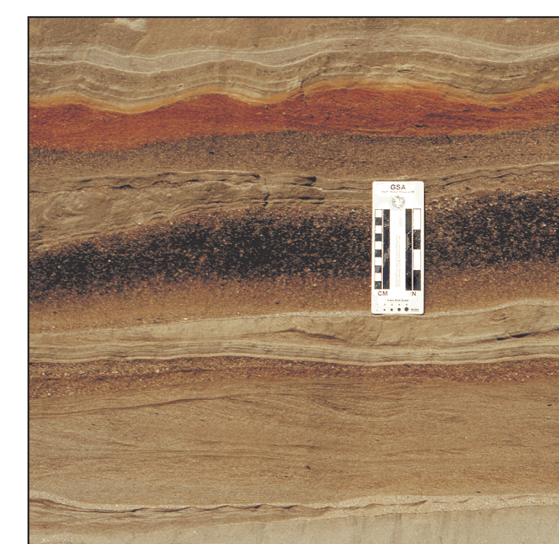
Sand (ranging from very fine-grained to very coarse): vfs-vcs -- Close-up of pit face in well-stratified sand beds deposited in glacial lake at lower end of Bear River valley, Newry.
