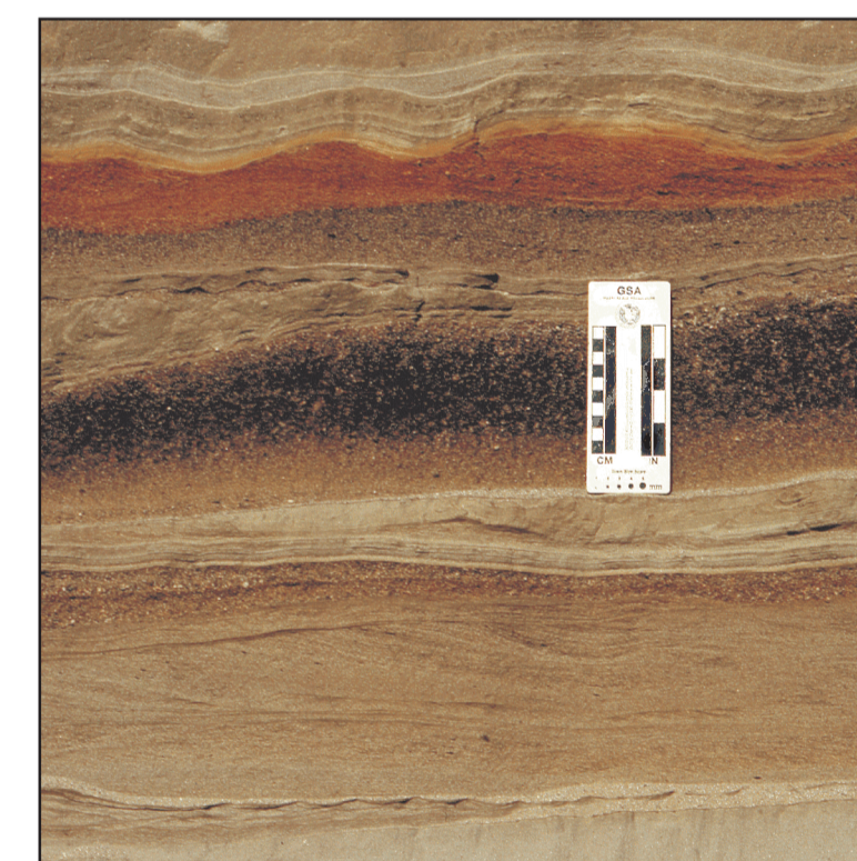
Sand (ranging from very fine-grained to very coarse): vs/vcs -- Close-up of pit face in well-stratified sand beds deposited in glacial lake at lower end of Bear River valley, Newry.
