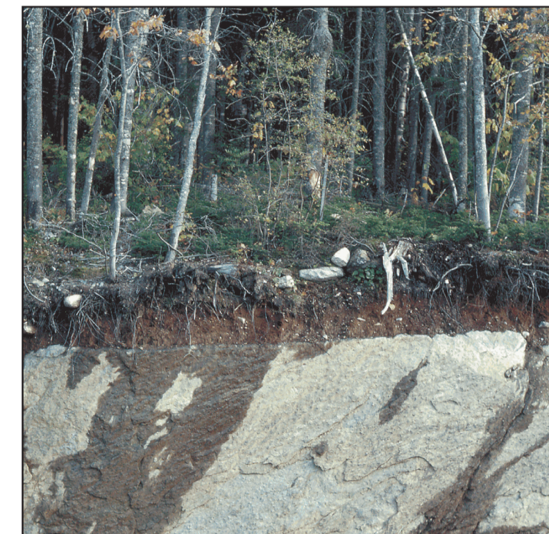
Till over bedrock: d(t)/rk -- Road cut on Route 17 in Township D, showing thin layer of till overlying glacially eroded bedrock. Dark streaks on the rock face are wet areas.
