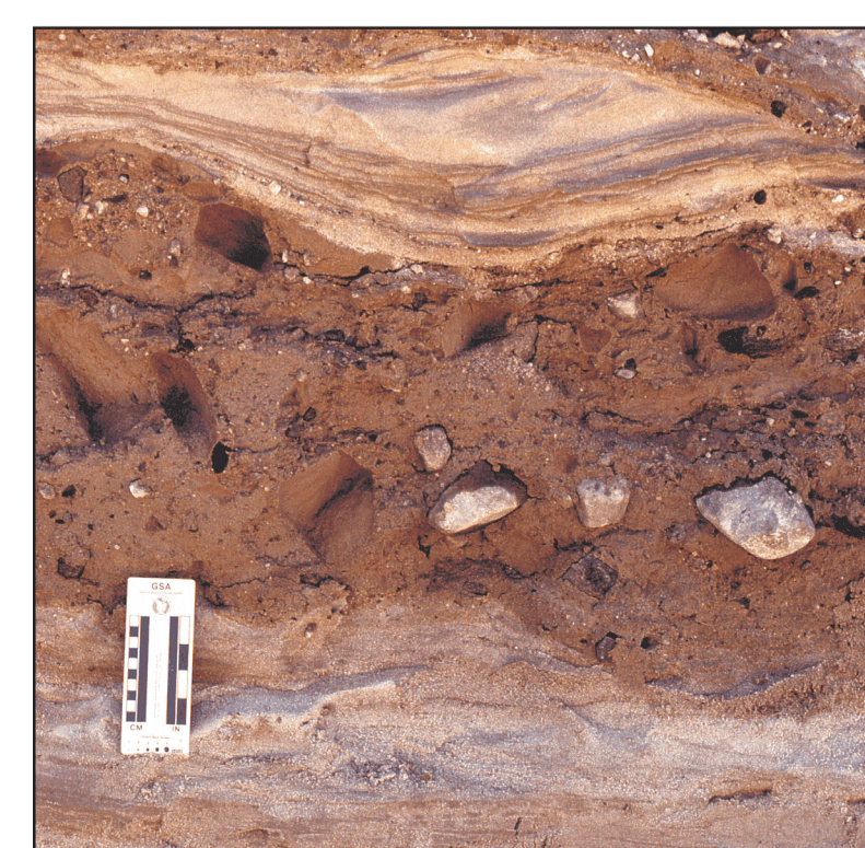
Sand with interbedded flowfill: s-ds(tf) -- Close-up of pit face in an end-moraine, Westbrook, showing part of a stony flowfill lens (center) deposited where glacial margin terminated in the sea.
