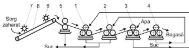
Fig. 7 - Scheme of the technological line for squeezing the juice from the sorghum strains, [1]
