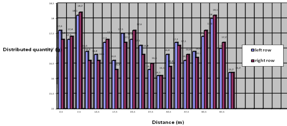
Fig. 3. Longitudinal distribution diagram achieve by the machine in conditions of test I, for the height of the samples test of 0,4 m.
