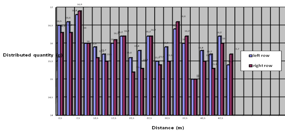
Fig. 3. Longitudinal distribution diagram achieve by the machine in conditions of test I, for the height of the samples test of 0,4 m.
