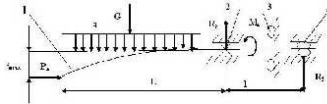
Fig. 2. Loading scheme of the shaft [2,4]
