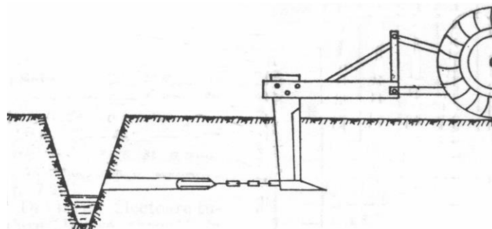
Figure 9 - Execution of mole drainage simultaneously with deep soil loosening, on a landscaped land with drainage channel
