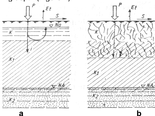
Figure 7 – The effect of deep soil loosening on land with hard permeabil clay layer located at small depth a – before soil loosening; b – after soil loosening
