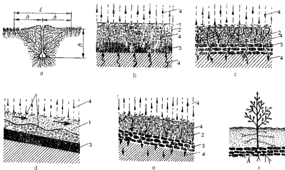
Figure 10 - The working process of the machines for deep soil loosening:
