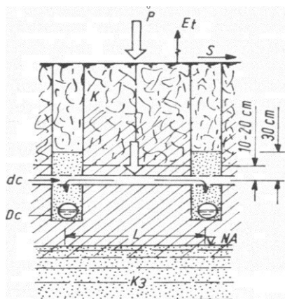
Figure 8 - The effect of deep soil loosening on land with hard permeabil clay layer of large thickness (after soil loosening and drainage)
