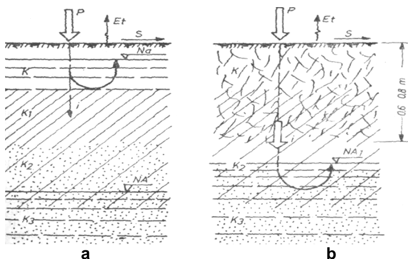
Figure 6 – The effect of deep soil loosening on land with hard permeabil clay layer located at small depth a – before soil loosening; b – after soil loosening
