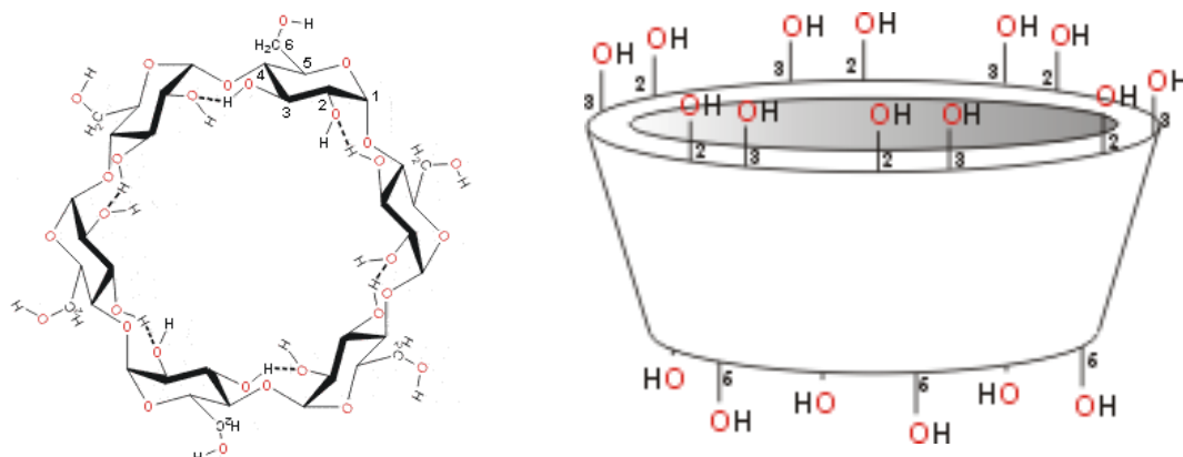
Figure 1 Cyclodextrins structure (Szejtli, 1982)
