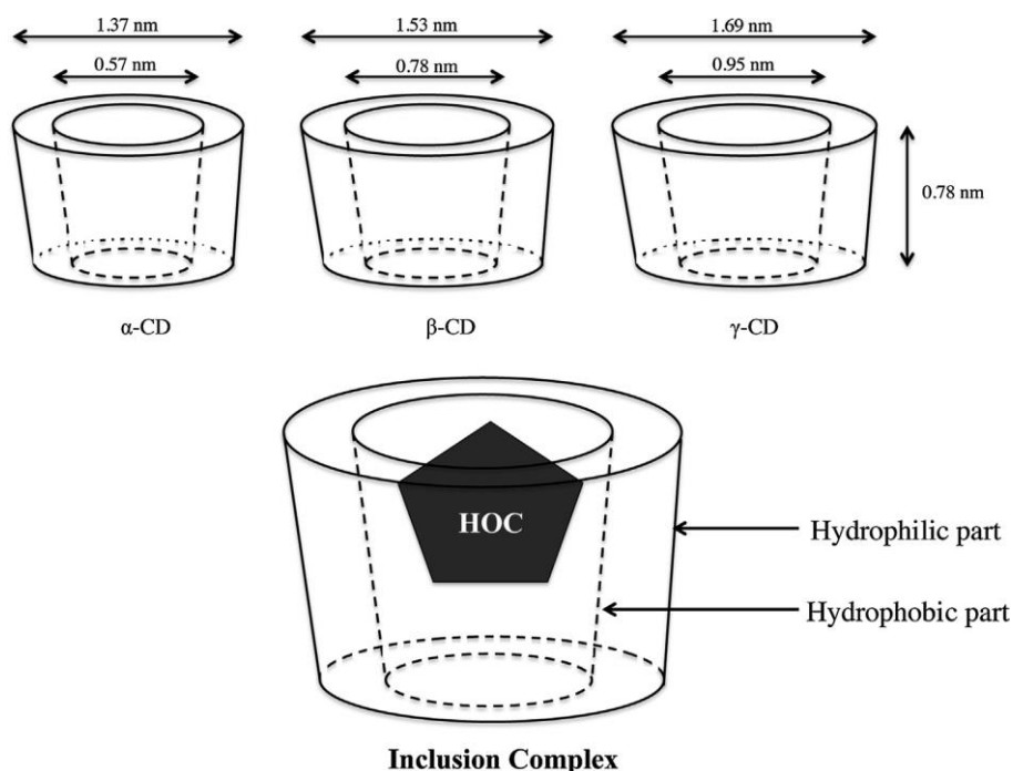
Figure 3 Structure of native cyclodextrins and inclusion complex formed with petroleum hydrocarbons (HOC) (Trellu si colab., 2016)
