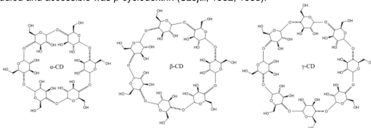
Figure 2 Structure of \alpha -, \beta - and \gamma -cyclodextrins (Szejtli, 1982)
