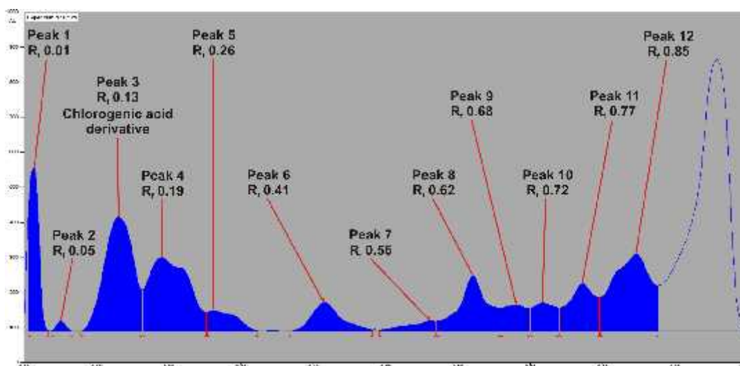
Figure 9. Densitogram of polyphenols (UV 254 nm) separated from Hyperici hirsuti herba methanolic extract.
