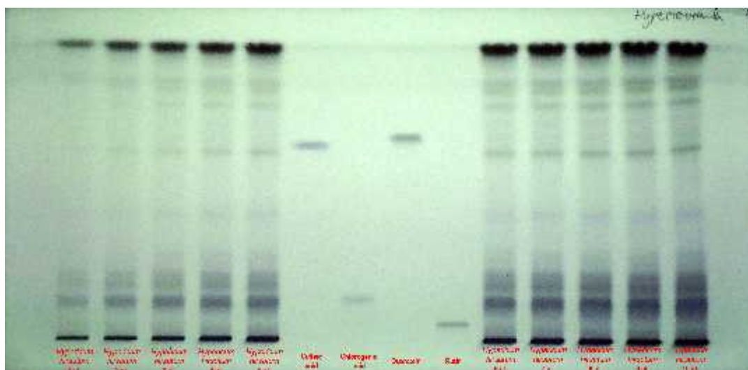
Figure 8. TLC chromatogram of polyphenols from Hyperici hirsuti herba methanolic extract (UV 254 nm, without derivatization). From left to right: first five applications – sample (1–5 µL); subsequent four applications – standards (2 µL); last five applications – sample (6–10 µL).
