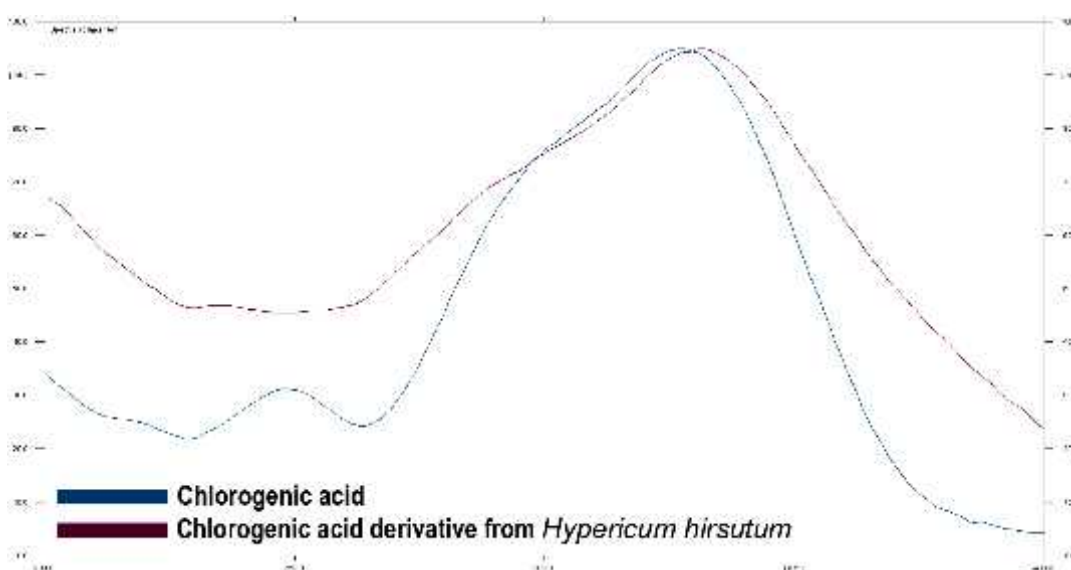
Figure 10. Chlorogenic acid derivative in situ UV spectra of standard and compound separated from the analyzed sample.
