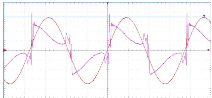
Gambar 3. Gelombang output induction heater
