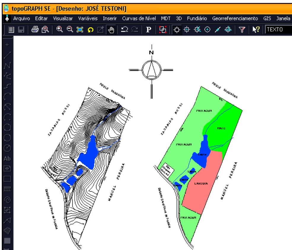
Figura 7 – Software topoGRAPH (2007).
